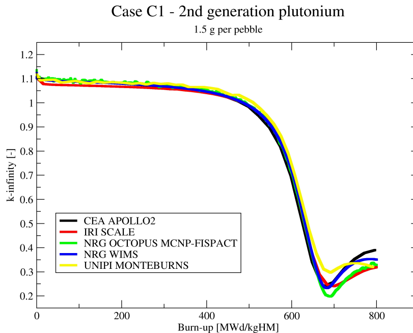
Fig. 1 Infinite multiplication factor as function of burnup (2nd generation Pu, 1.5 g).
