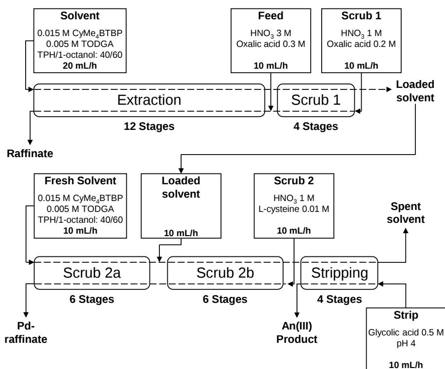
Figure 9: 1-cycle SANEX process flow-sheet.
