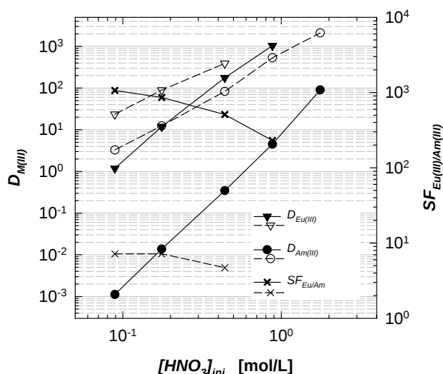
Figure 5. Effect of SO 3 -Ph-BTP on the extraction of Am(III) and Eu(III) into TODGA.
