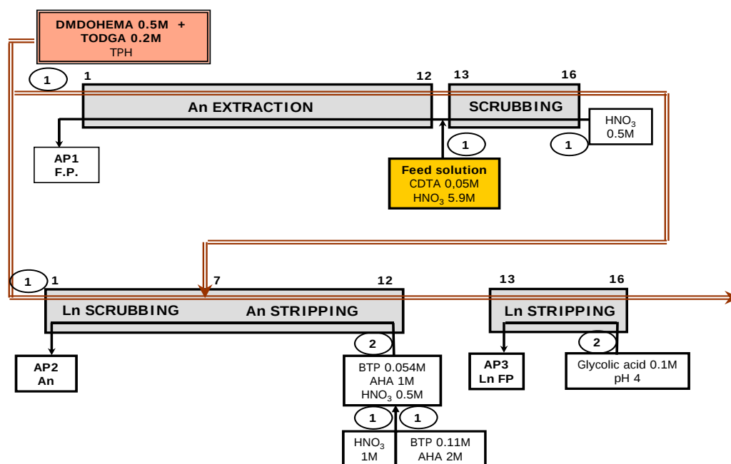
Figure 11. EURO-GANEX flow-sheet for the hot test.
