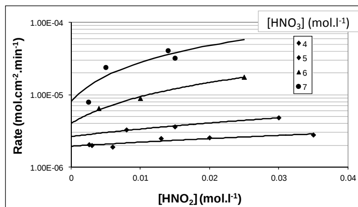
Figure 1: Linear dissolution rate constant for 4.7 % Pu \text{MOx} powder, effect of nitric acid and nitrous acid.
