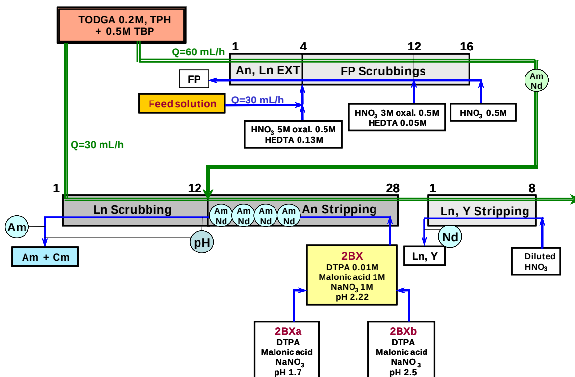
Figure 10: Optimized process flowsheet for the i -SANEX hot test.
