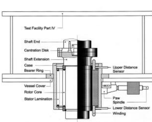
Fig 5. FLP500 test facility
