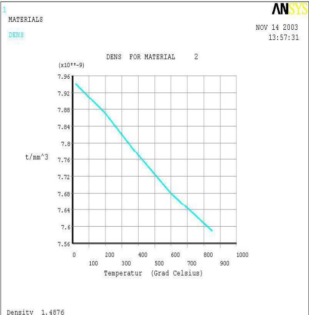
Figure 2-6: Density Alloy 800H
