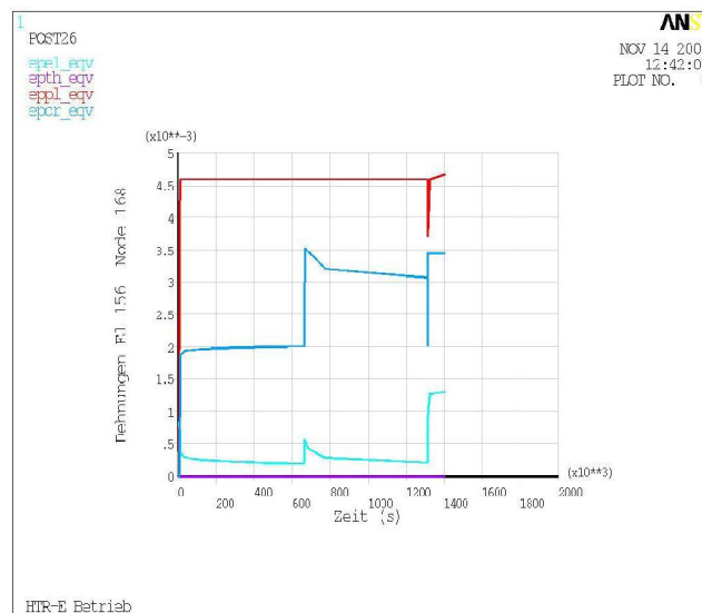
Figure 3-11: Equivalent Strains at Node 168
