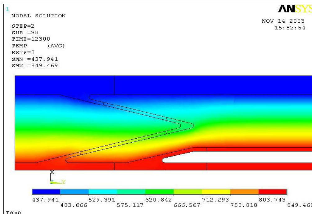
Figure 3-4: Temperature Distribution at 12300 sec. - 3,4 h after start up (Normal Operation)
