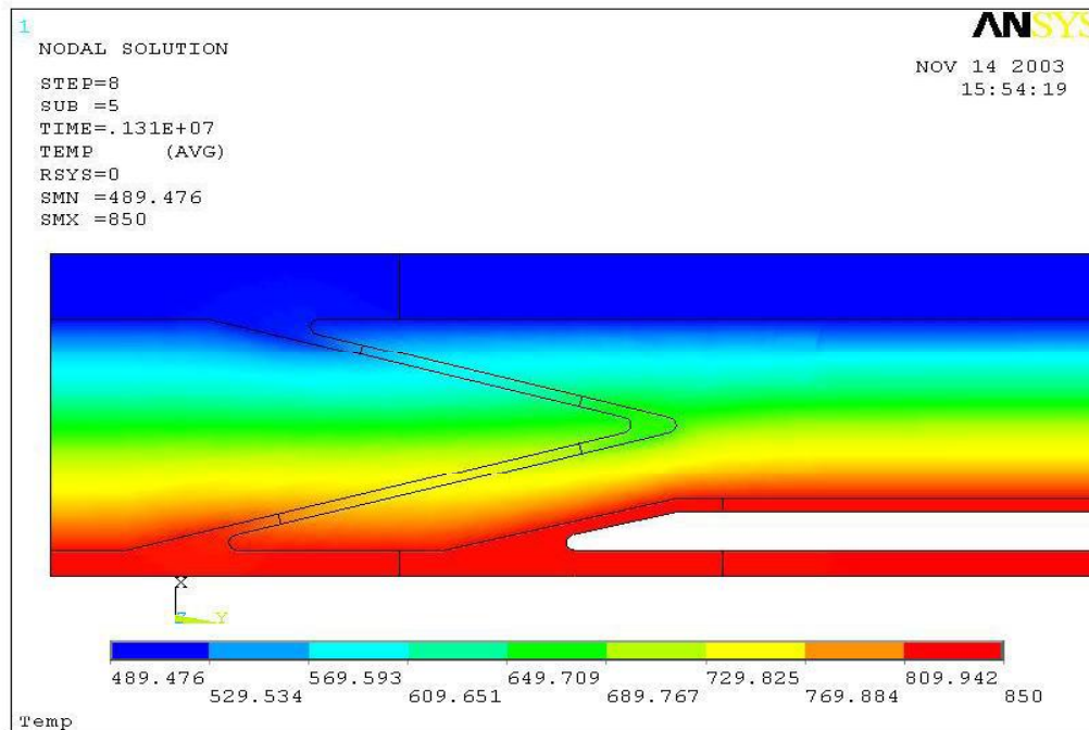
Figure 3-5: Temperature Distribution at 131E+7 sec.
