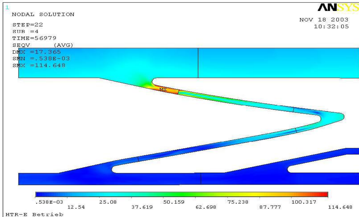
Figure 3-8: Equivalent Stress during Normal Operation for the Model with Different Material
