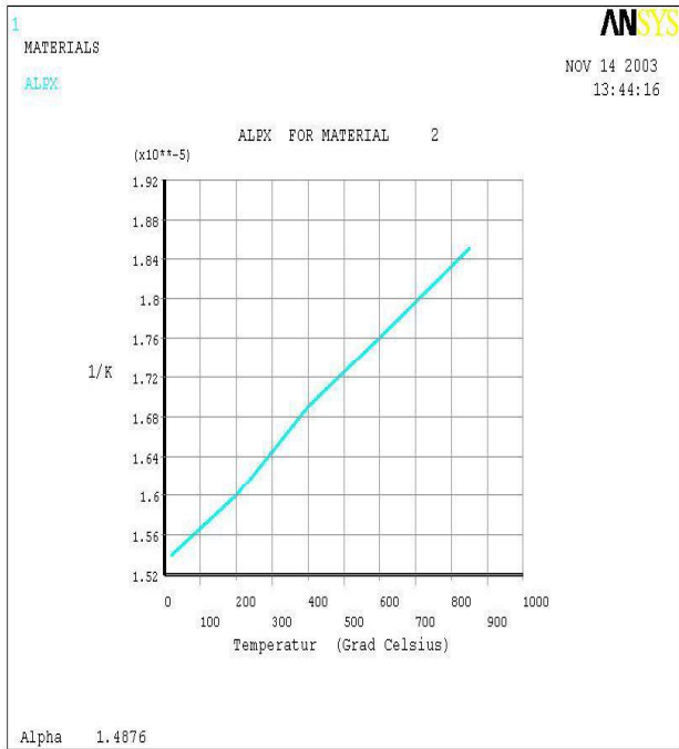
Figure 2-4: Thermal Expansion Coefficient Alloy 800H
