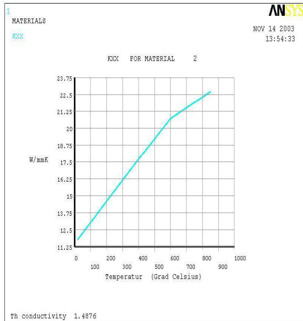
Figure 2-10: Thermal Transfer Coefficient Alloy 800H
