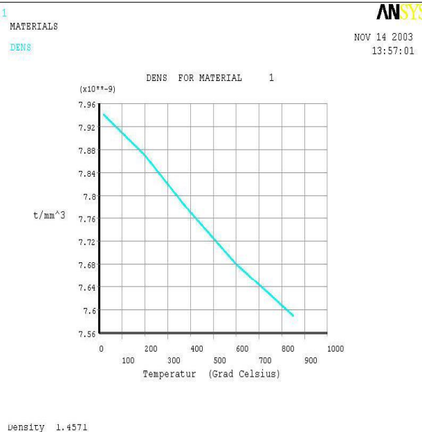
Figure 2-5: Density 1.4571
