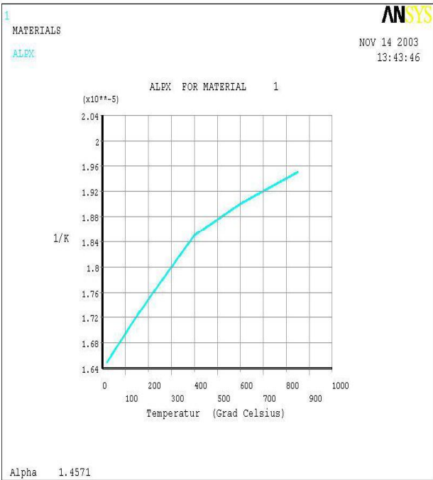
Figure 2-3: Thermal Expansion Coefficient 1.4571
