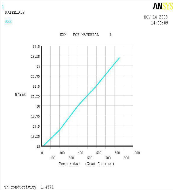
Figure 2-9: Thermal Transfer Coefficient 1.4571
