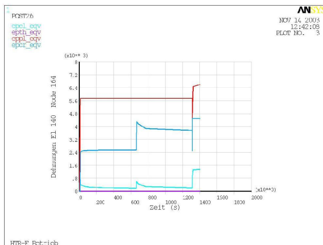
Figure 3-9: Equivalent Strains at Node 164
