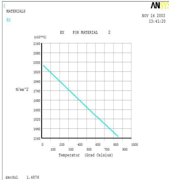
Figure 2-8: E-Module Alloy 800H
