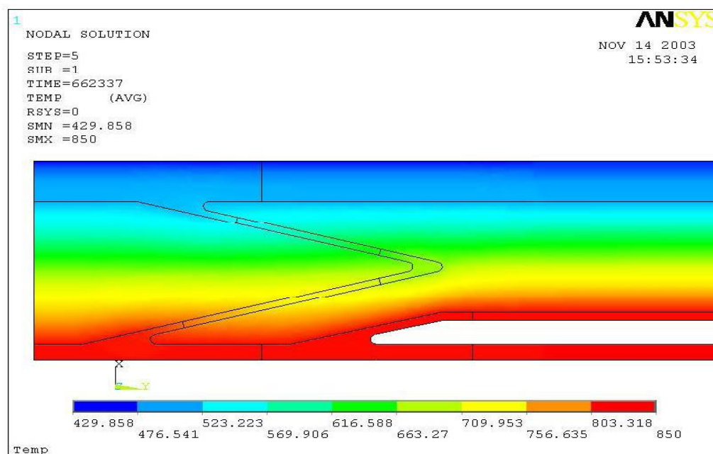
Figure 3-3: Temperature Distribution at 662337 sec (Normal Operation) Cold shock at the outside of the support tube with 60K/sec.
