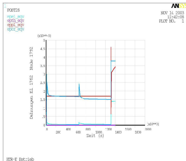
Figure 3-12: Equivalent Strains at Node 1792
