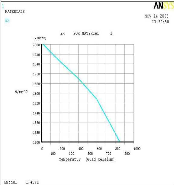
Figure 2-7: E-Module 1.4571
