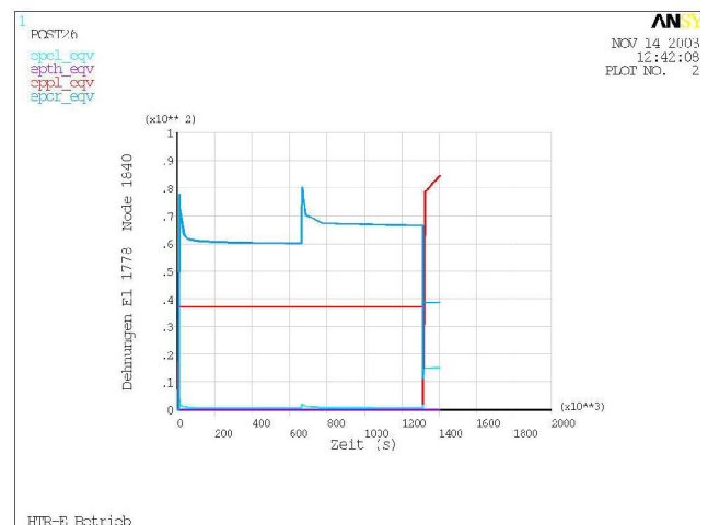
Figure 3-10: Equivalent Strains at Node 1840
