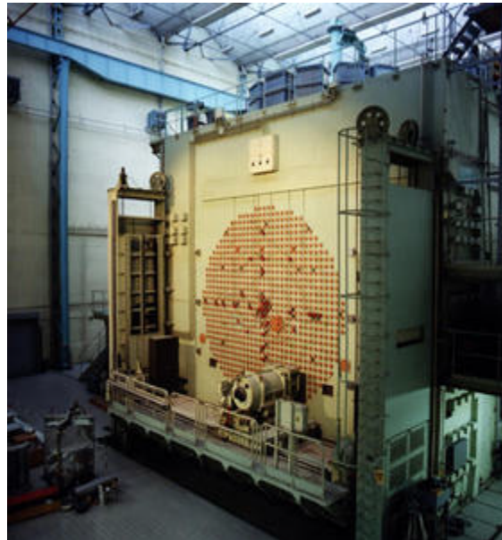
Figure 1: BR-1 Reactor 3
