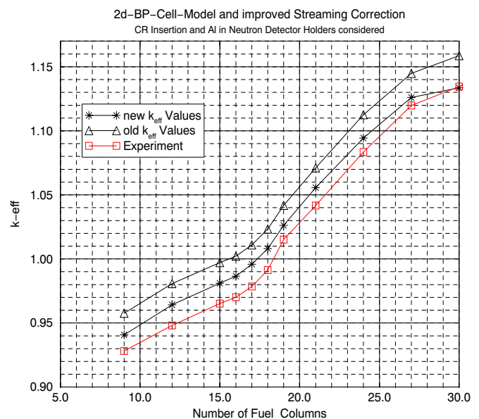
Fig.1: New and Old k_{eff} -Values of the Diffusion Calculations in Comparison with the Experiment
