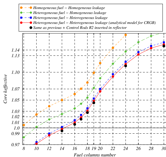
Fig 2. k_{\text{eff}} -values obtained by different core models
