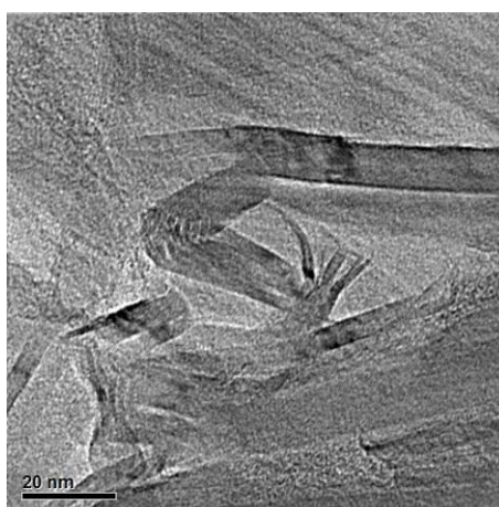
Figure 8: TEM photographs of EG from S20H1 showing the graphene layers separation at different scales.
