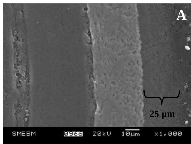
Figure 4: Representative SEM crosses sections of TRISO particles (embedded into a resin) after MW treatment (A) and RT treatment (B), showing the oxidation of the OPyC layer during the MW treatment.
