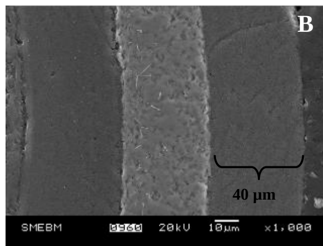
Figure 4: Representative SEM crosses sections of TRISO particles (embedded into a resin) after MW treatment (A) and RT treatment (B), showing the oxidation of the OPyC layer during the MW treatment.
