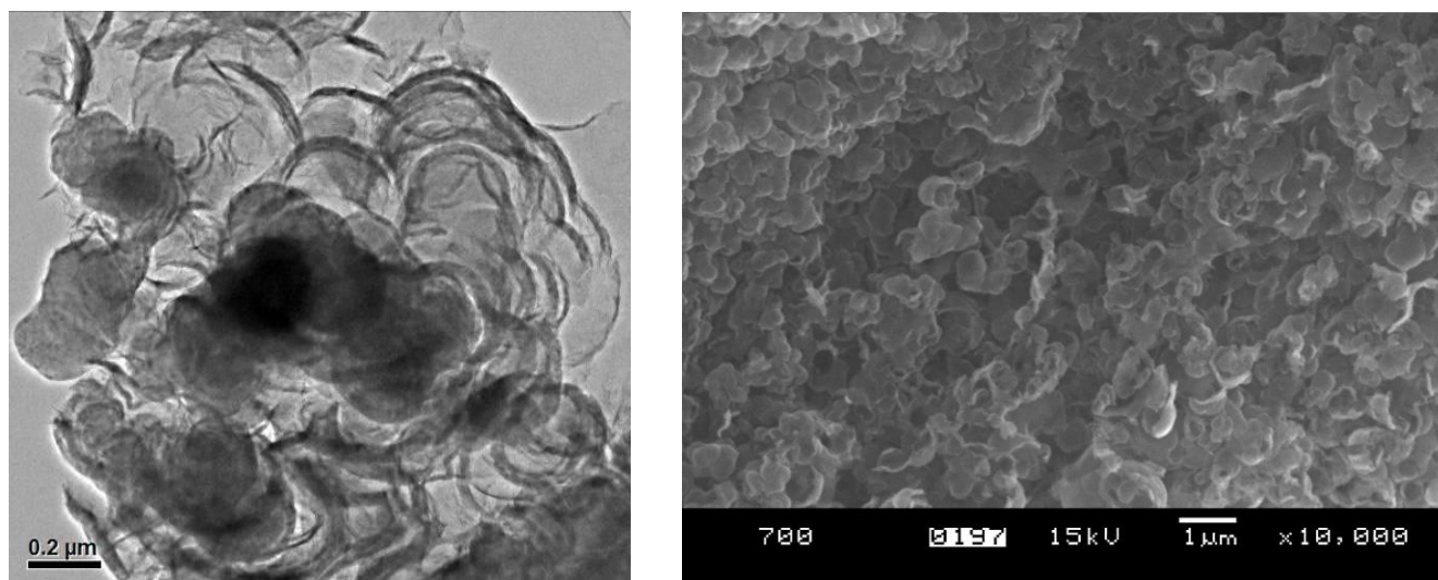
Figure 5: TEM and SEM photographs of OPyC after a MW treatment (from S7N3) showing a particle size between 200 and 400 nm.
