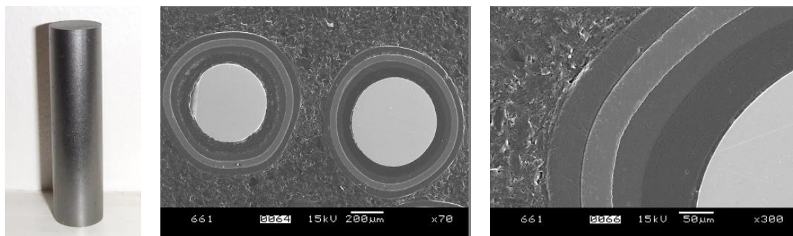
Figure 1: Graphite compact (left) in which TRISO particles (centre, right) are embedded.
