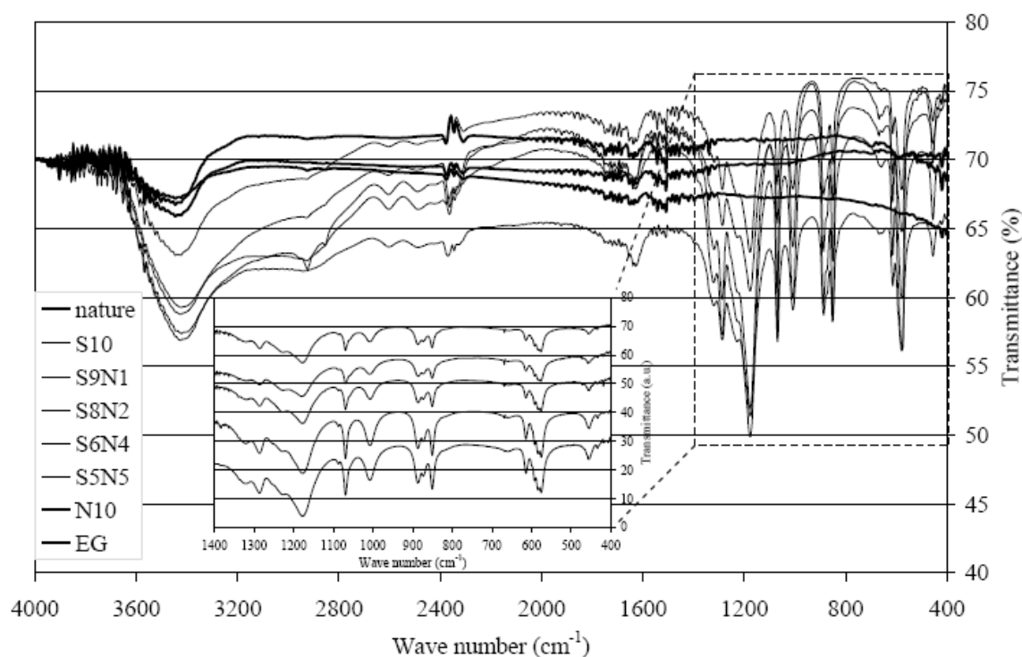
Figure 2: Infrared spectra of rinsed H_2SO_4 -GICs prepared by microwave, compared with natural graphite and exfoliated graphite. In medallion is represented a zoom of the “digital prints” region 400-1400 cm^{-1} where appear sulfur bands.
