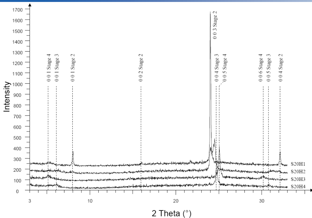
Figure 7: X-ray diffractograms of H 2 SO 4 -GICs prepared in mixtures of H 2 O 2 /H 2 SO 4 at RT, showing different stages depending on this volume ratio. Step: 0.02°, Step time: 2 s.
