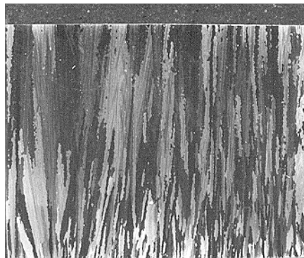
Figure 20 : General view of CM 247 test bar microstructure (specimen width=16 mm)
