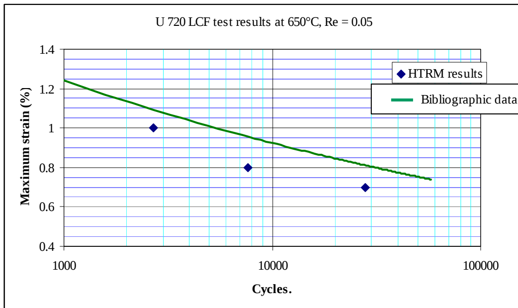
Figure 19 : Comparison of the LCF strength for HTRM U720 forged material with bibliographic data found in [Burlet03].
