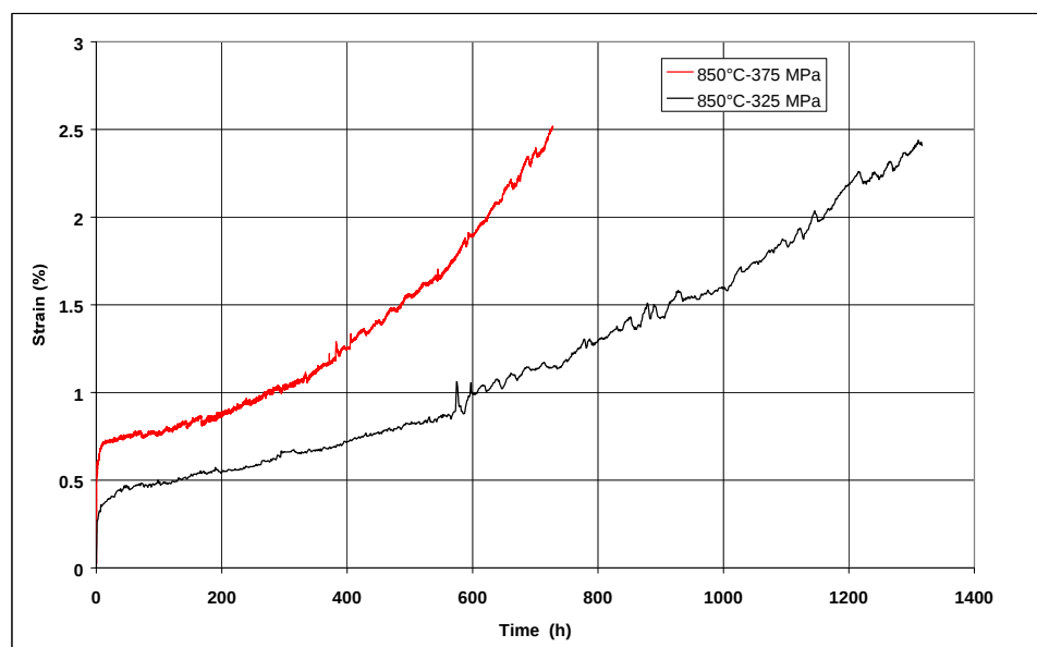
Figure 26 : Intermediate creep results obtained in November 2003 for CM 247 LC DS grade at 850°C.
