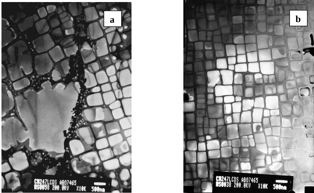
Figure 23 : General TEM view of CM 247 LC DS structure.
