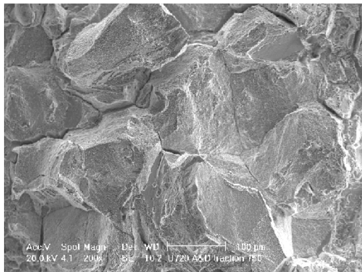
Figure 9 : SEM observation of a KCV impact toughness specimen broken at 20°C.
