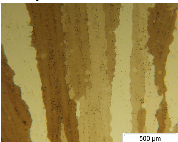
Figure 20 : General view of CM 247 test bar microstructure (specimen width=16 mm)
