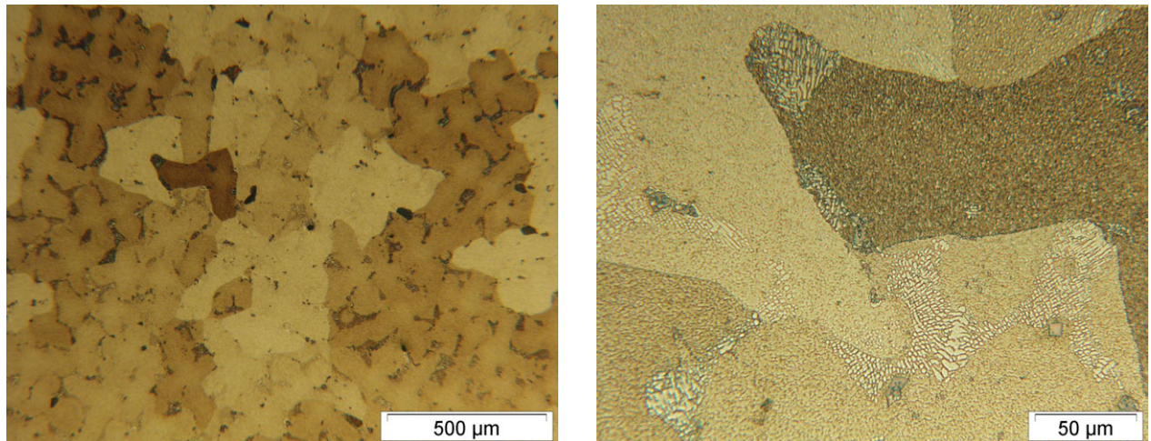
Figure 22 : Microstructure of CM 247, transverse orientation, at low and high magnifications.
