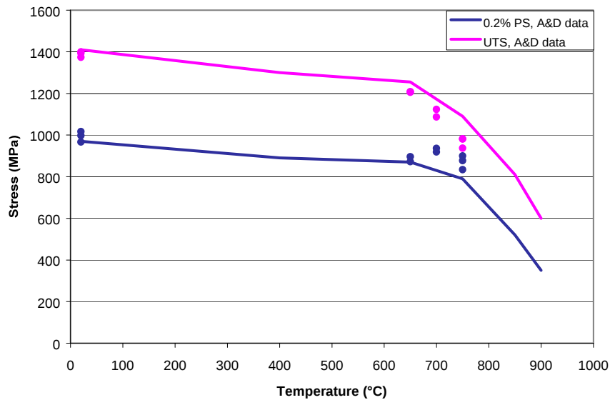
Figure 8 : HTRM Tensile results on forged U720 compared with A&D data.
