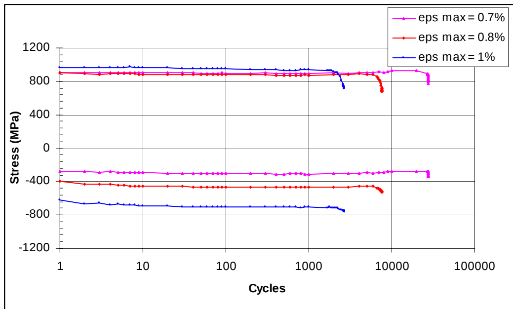
Figure 18 : Stress versus cycle number for U720 LC tested in LCF at 650°C.
