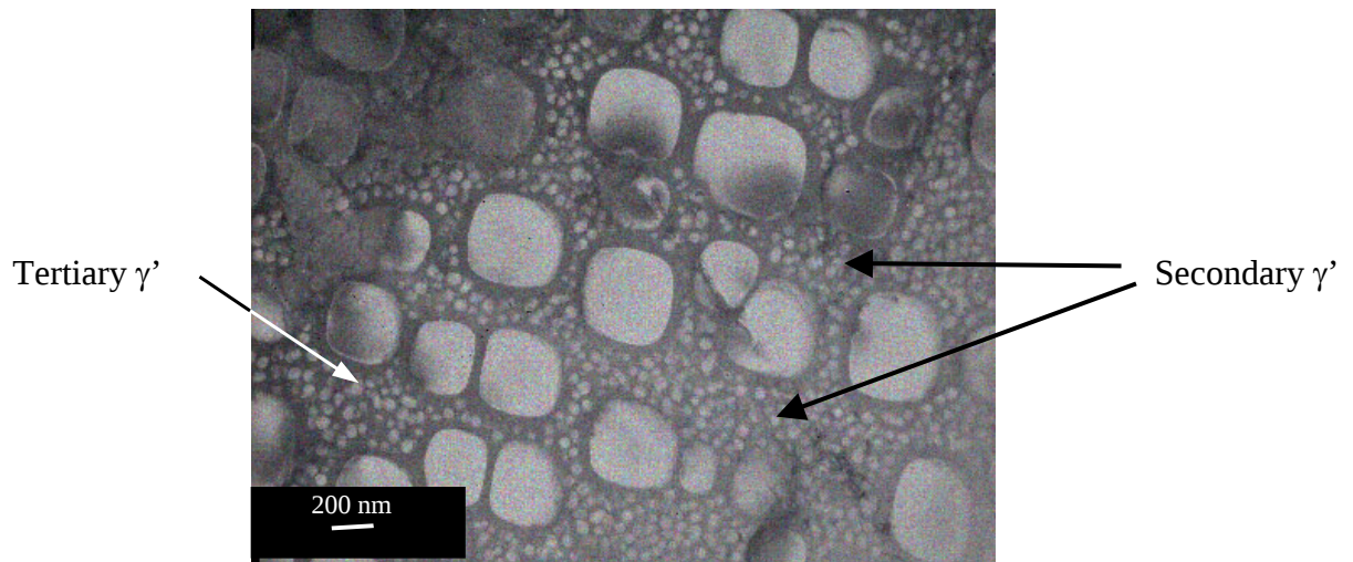
Figure 5 : TEM observation of the smallest \gamma' precipitates.
