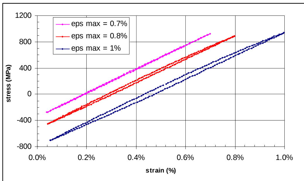
Figure 17 : Stress-Strain curves of U720 LC tested in LCF at 650°C (plotted at cycle N_r/2 ).
