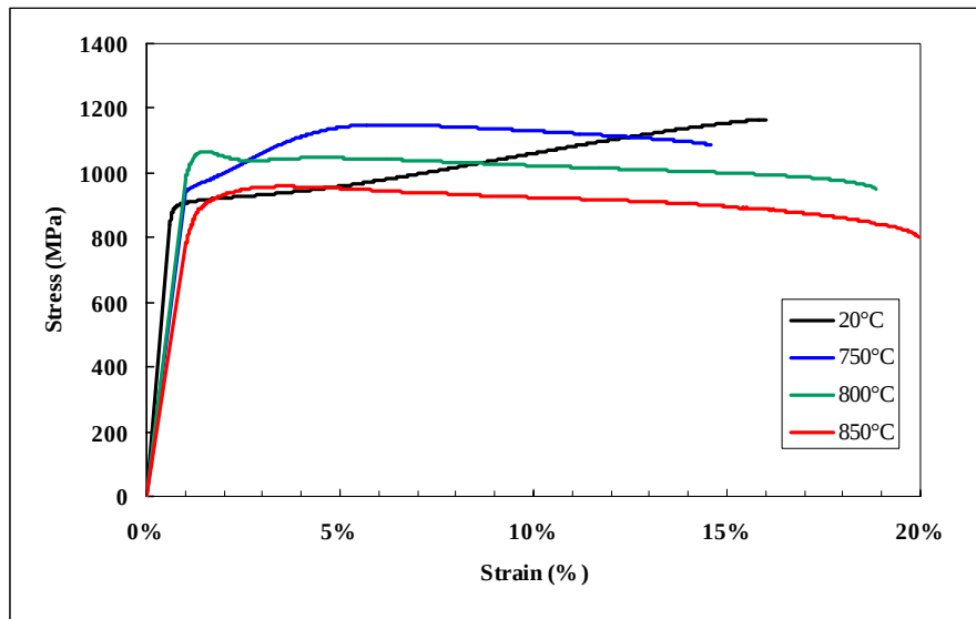
Figure 25 : Tensile stress/strain curves obtained on CM 247 LC DS material.
