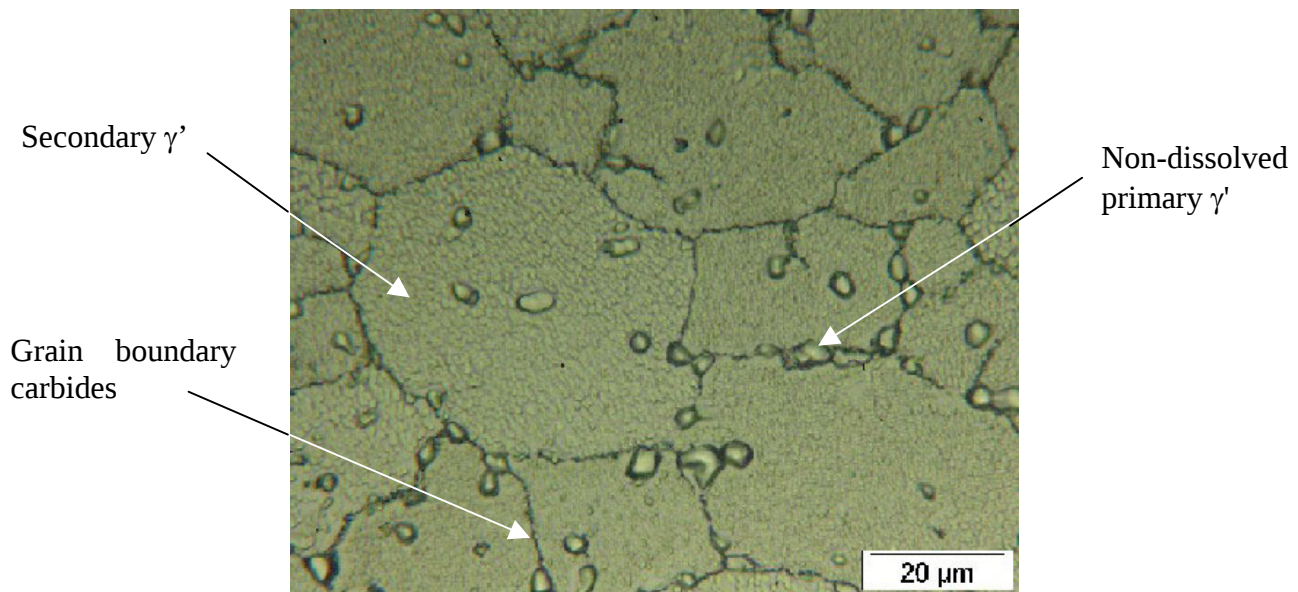
Figure 2 : General microstructure of forged U720.
