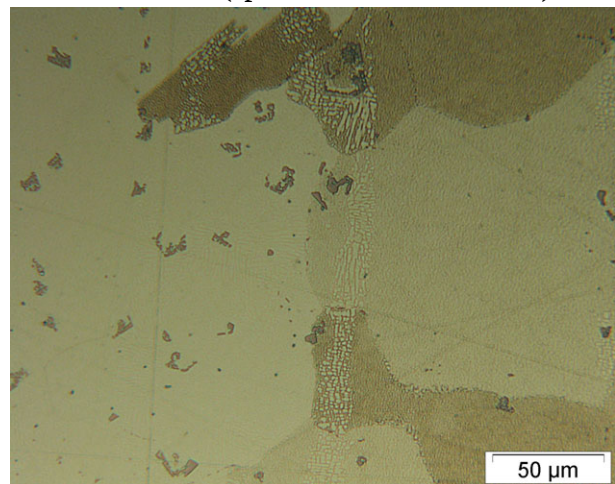
Figure 20 : General view of CM 247 test bar microstructure (specimen width=16 mm)
