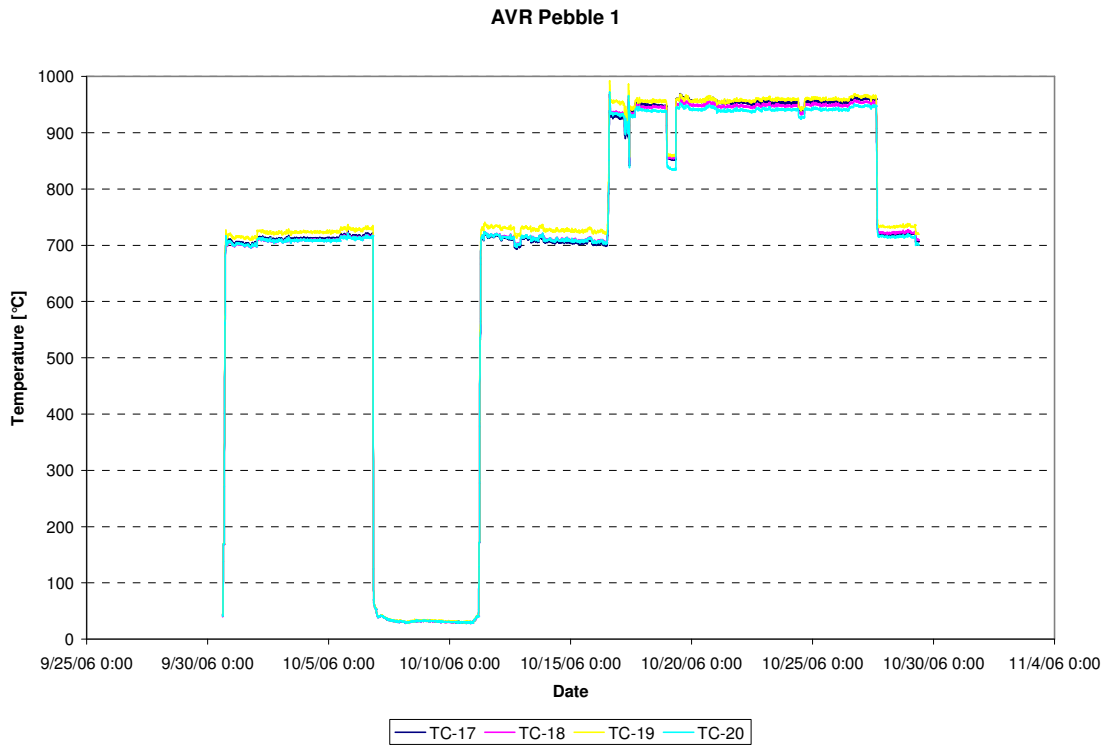
Figure 21: Temperatures pebble AVR.1 (TC-17, TC-18, TC-19, TC-20), cycle 06-08
