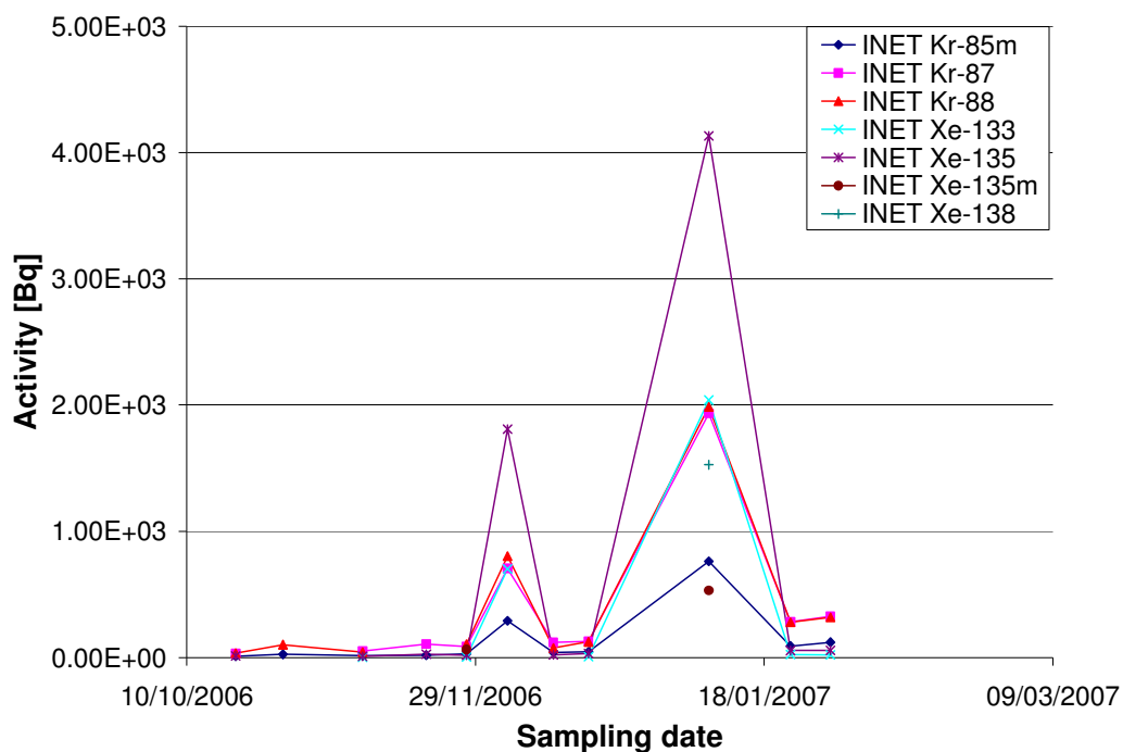
Figure 71: Release measurement vs. date for INET pebbles
