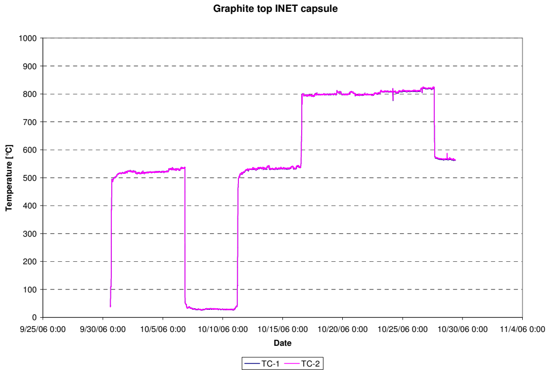
Figure 24: Temperatures top graphite INET capsule (TC-01, TC-02), cycle 06-08
