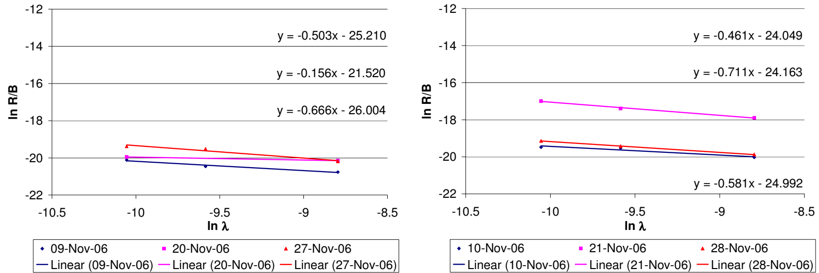
Figure 79: \ln R/B vs. \ln \lambda_{\text{eff}} plots for Krypton of INET/AVR pebbles in cycle 06-09
