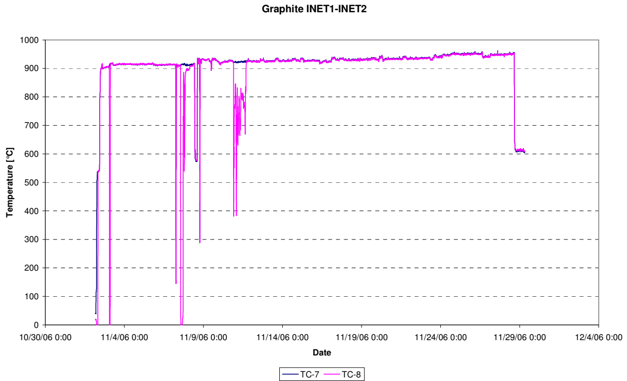
Figure 37: Temperatures graphite between INET.1 and INET.2 (TC-07, TC-08), cycle 06-09
