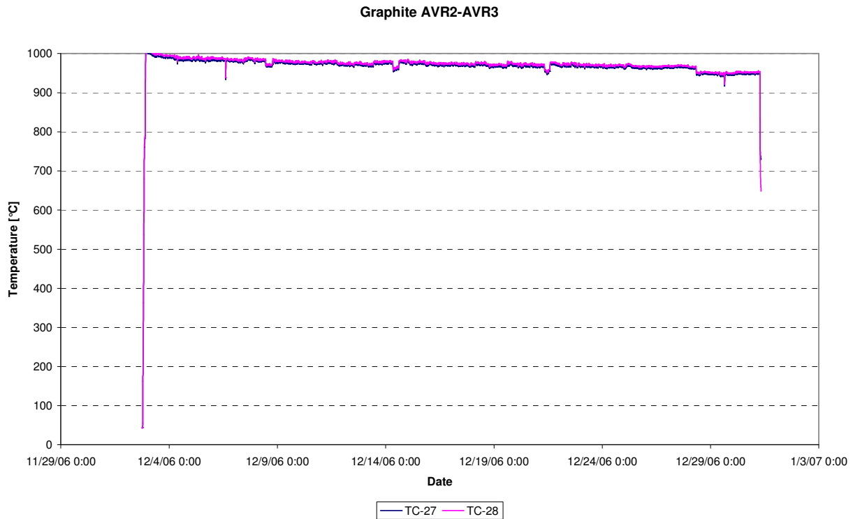
Figure 53: Temperatures graphite between AVR.2 and AVR.3 (TC-27, TC-28), cycle 06-10
