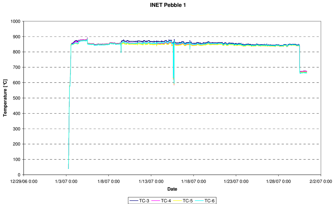
Figure 55: Temperatures pebble INET.1 (TC-03, TC-04, TC-05, TC-06), cycle 07-01
