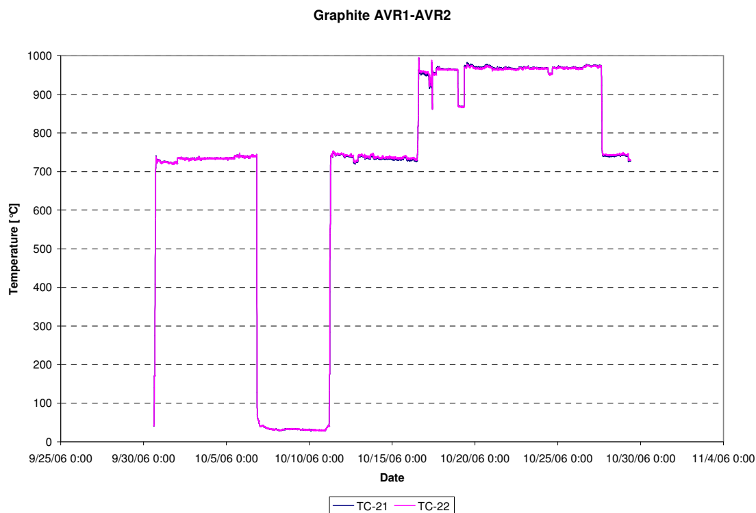
Figure 28: Temperatures graphite between AVR.1 and AVR.2 (TC-21, TC-22), cycle 06-08
