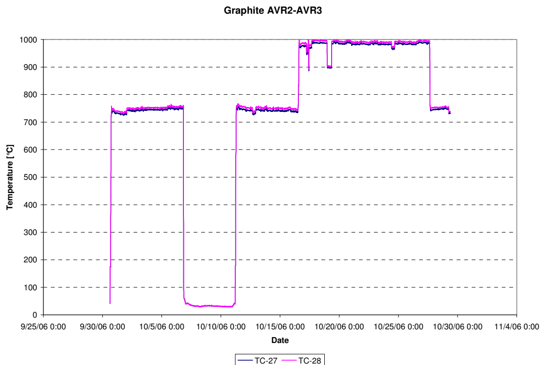
Figure 29: Temperatures graphite between AVR.2 and AVR.3 (TC-27, TC-28), cycle 06-08
