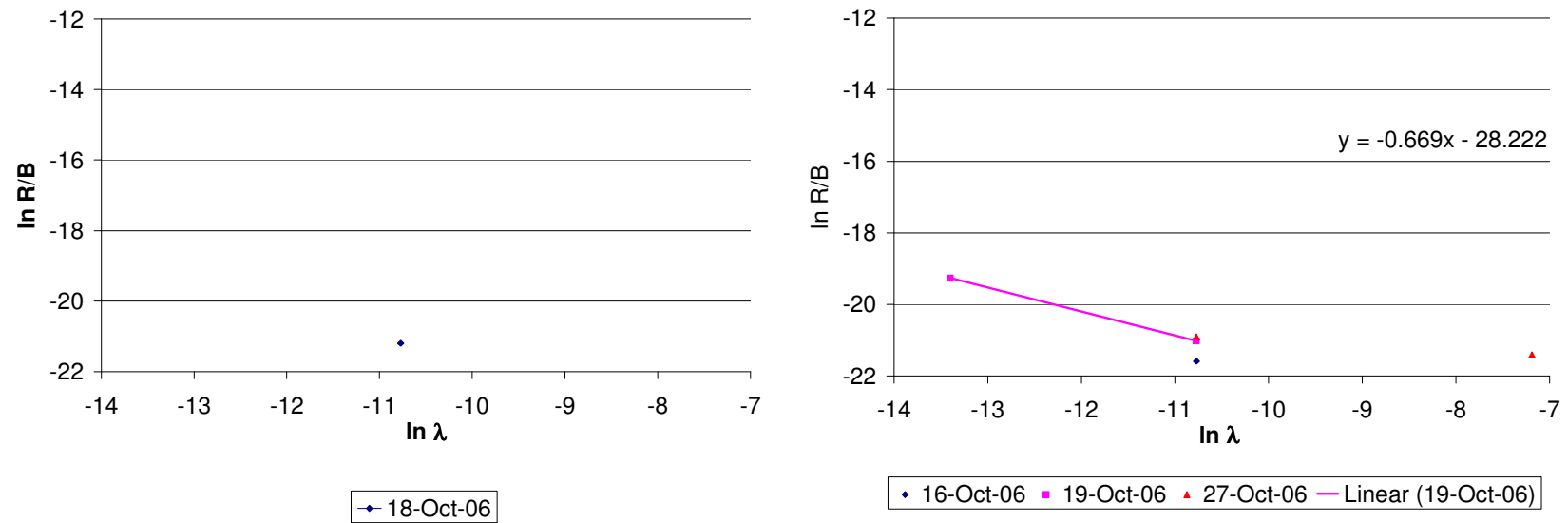
Figure 78: \ln R/B vs. \ln \lambda_{\text{eff}} plots for Xenon of INET/AVR pebbles in cycle 06-08
