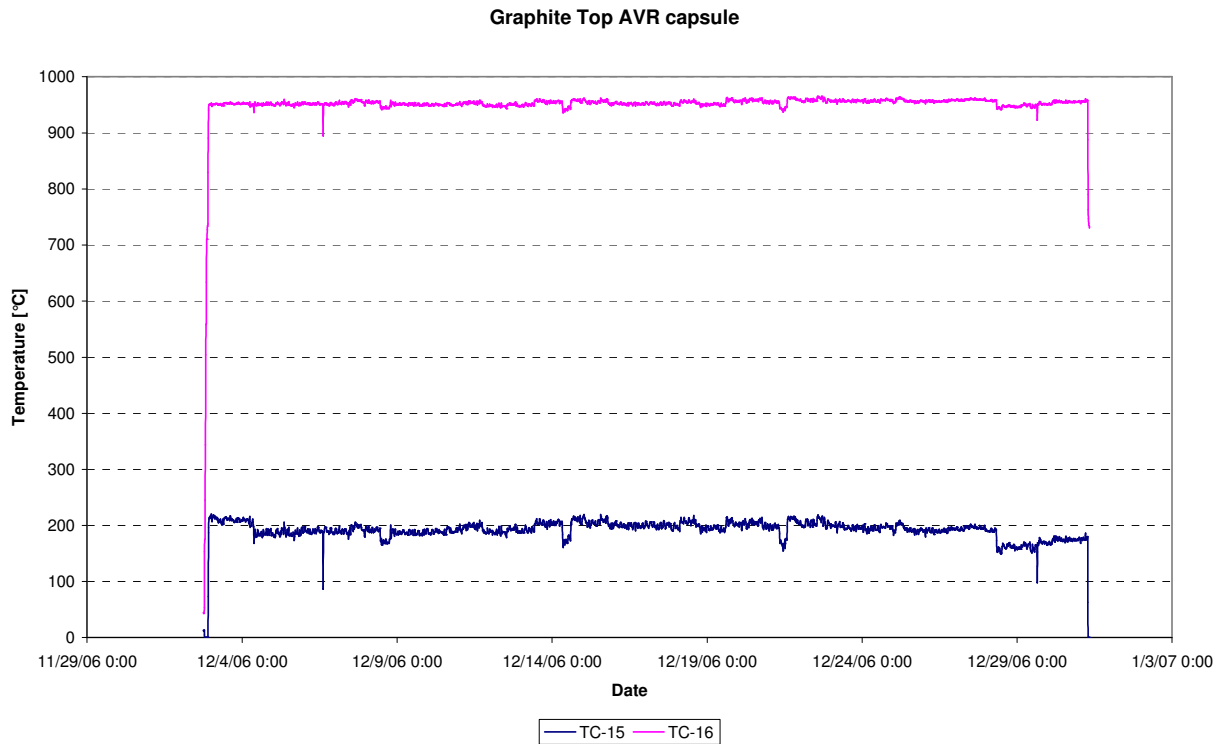
Figure 51: Temperatures top graphite AVR capsule (TC-15, TC-16), cycle 06-10
