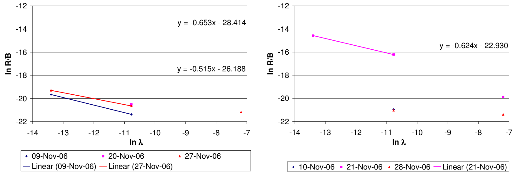
Figure 80: \ln R/B vs. \ln \lambda_{\text{eff}} plots for Xenon of INET/AVR pebbles in cycle 06-09
