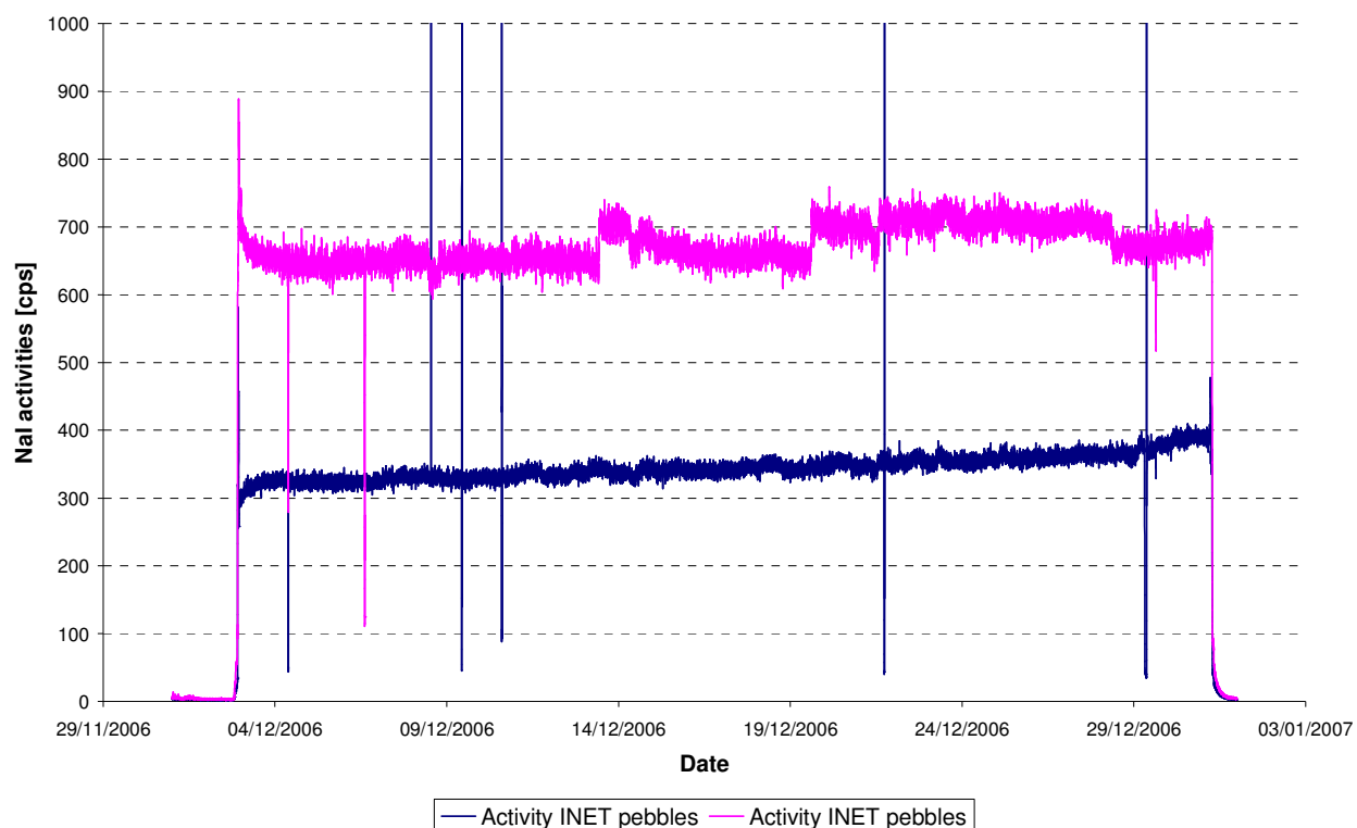
Figure 15: Nal readings cycle 06-10
