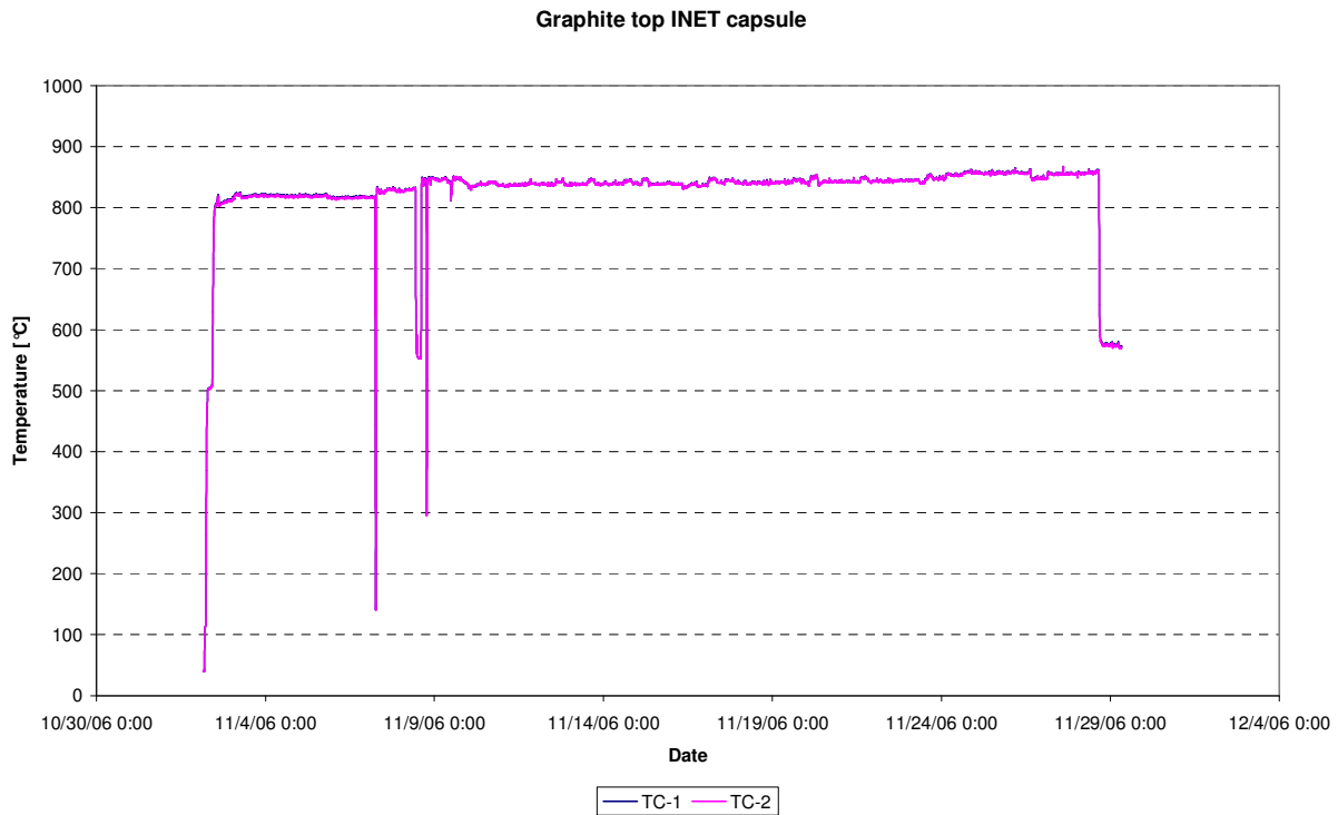
Figure 36: Temperatures top graphite INET capsule (TC-01, TC-02), cycle 06-09
