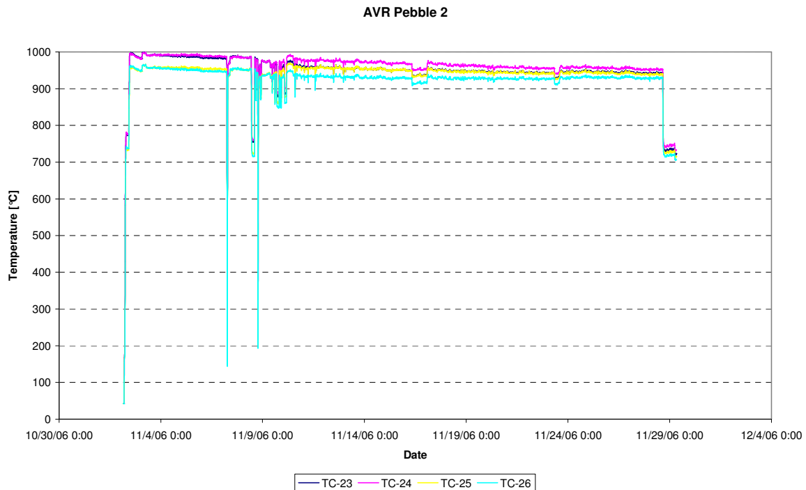
Figure 34: Temperatures pebble AVR.2 (TC-23, TC-24, TC-25, TC-26), cycle 06-09
