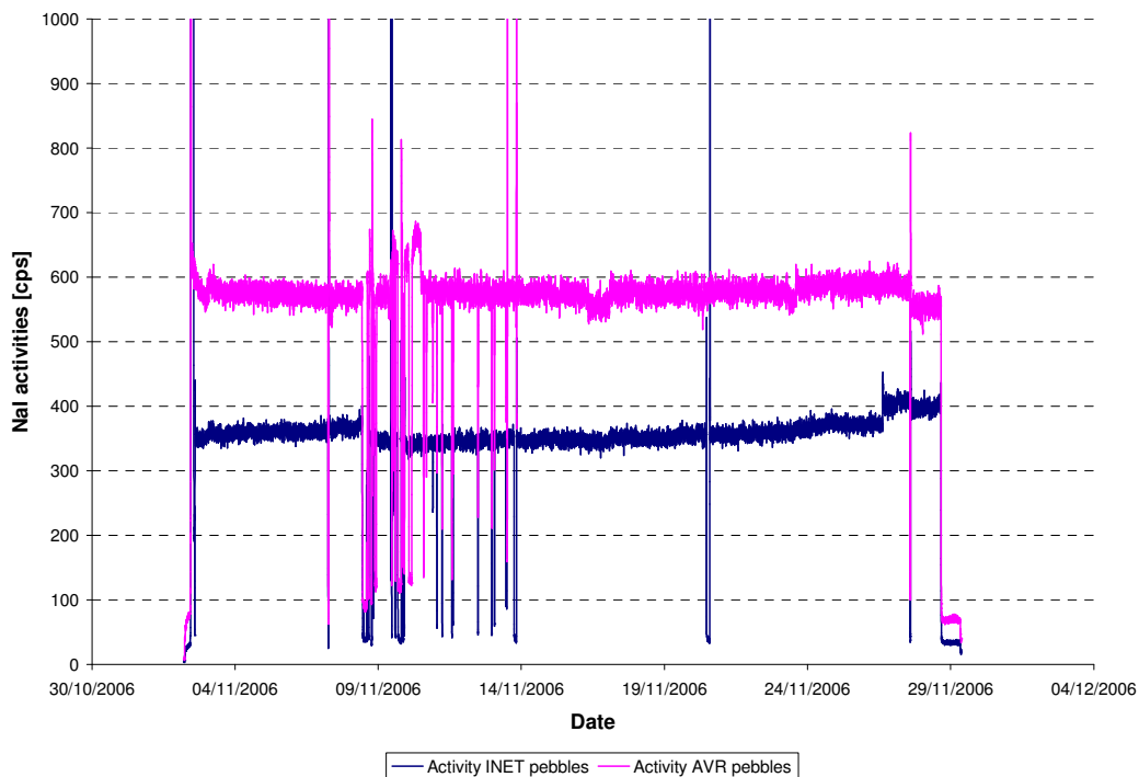
Figure 14: Nal readings cycle 06-09
