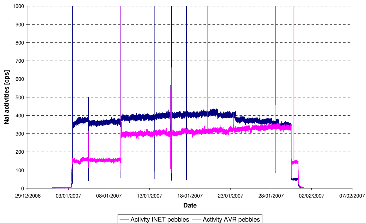
Figure 16: Nal readings cycle 07-01
