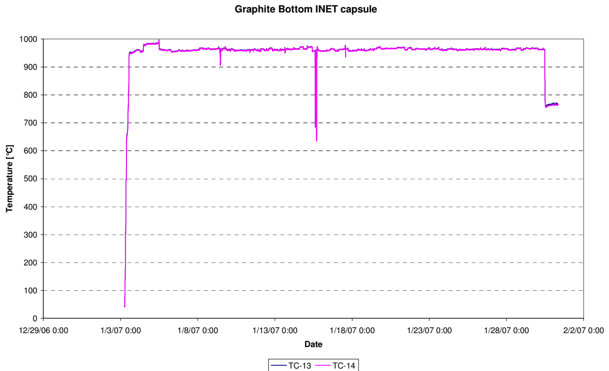
Figure 62: Temperatures bottom graphite INET Capsule (TC-13, TC-14), cycle 07-01
