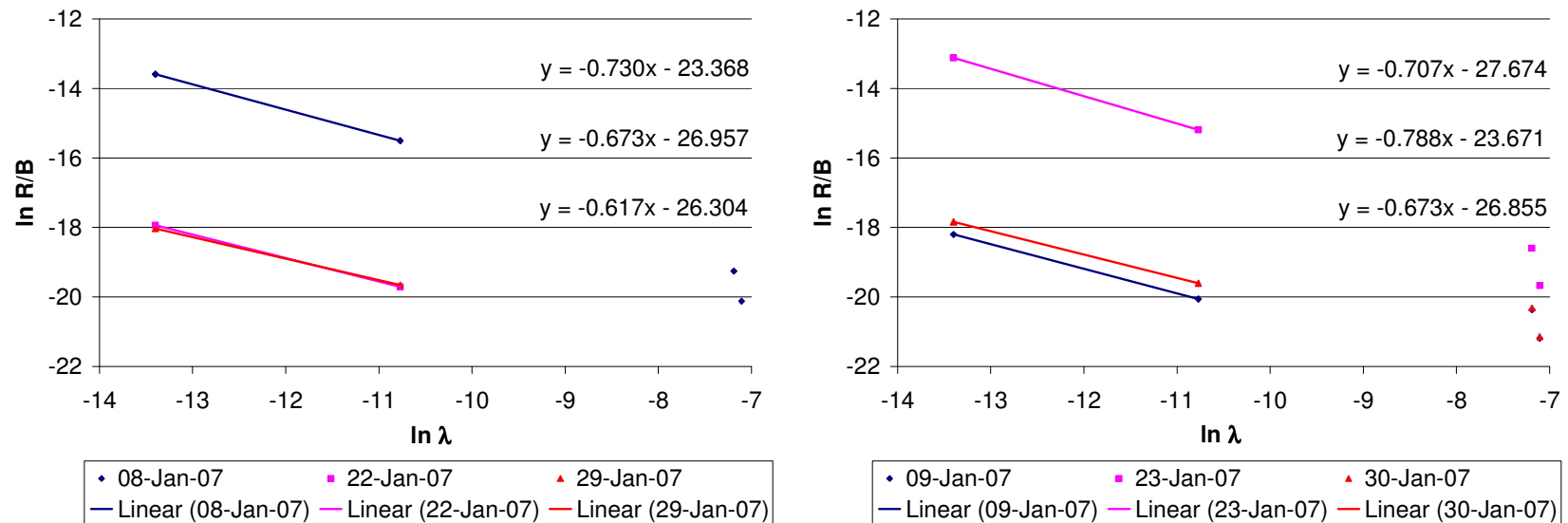
Figure 84: \ln R/B vs. \ln \lambda_{\text{eff}} plots for Xenon of INET/AVR pebbles in cycle 07-01
