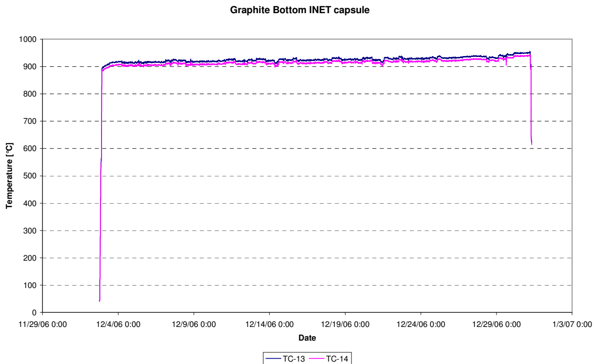
Figure 50: Temperatures bottom graphite INET Capsule (TC-13, TC-14), cycle 06-10
