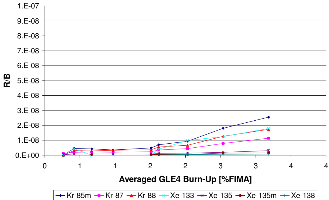
Figure 76: R/B vs. burnup for AVR pebbles
