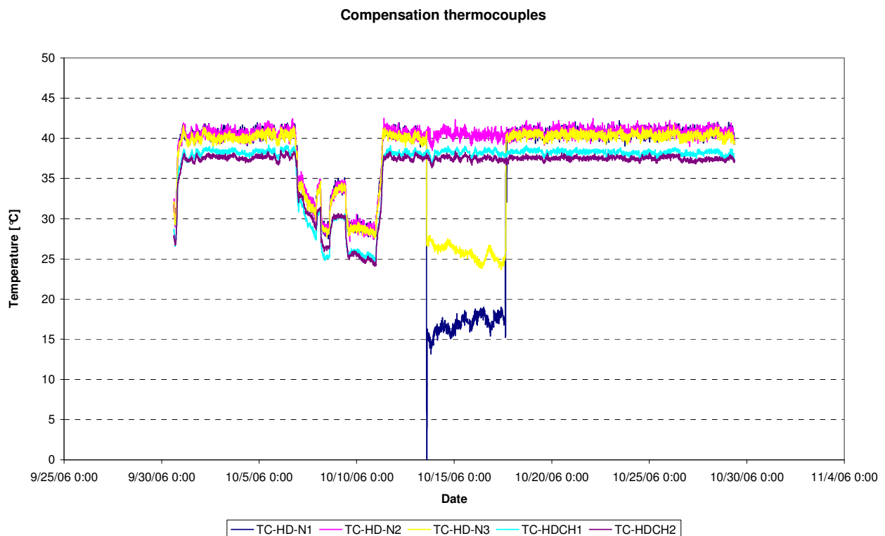
Figure 67: Reference thermocouples for temperatures compensation cycle 06-08
