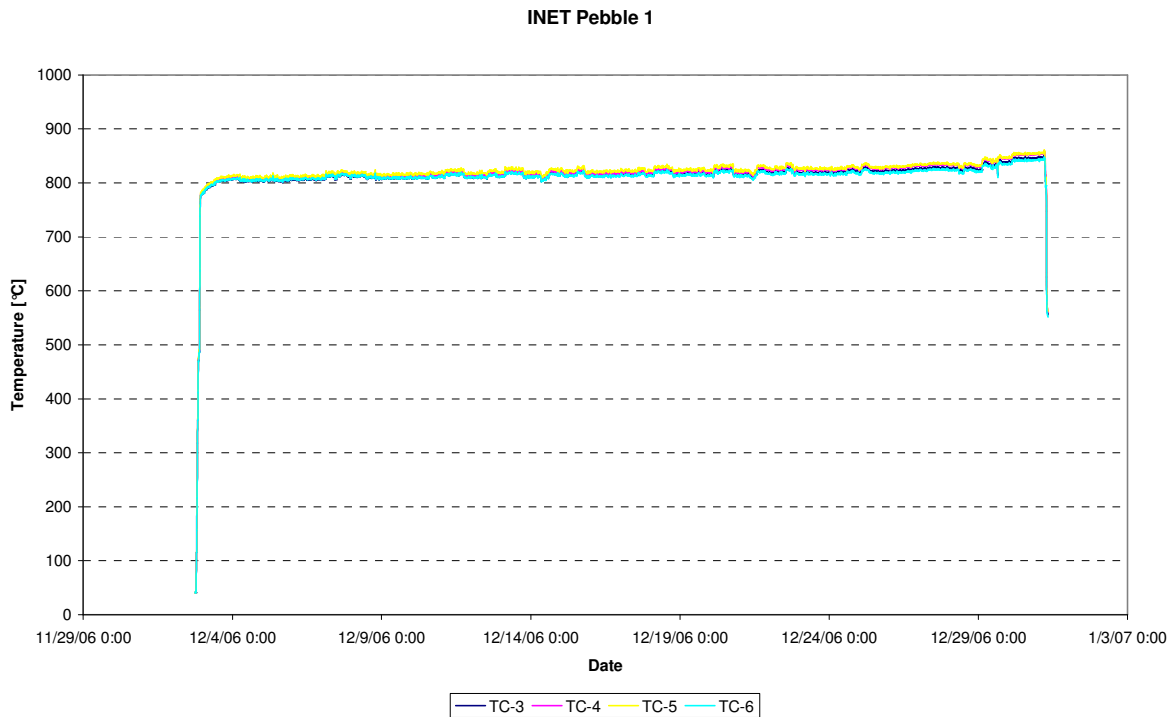
Figure 43: Temperatures pebble INET.1 (TC-03, TC-04, TC-05, TC-06), cycle 06-10
