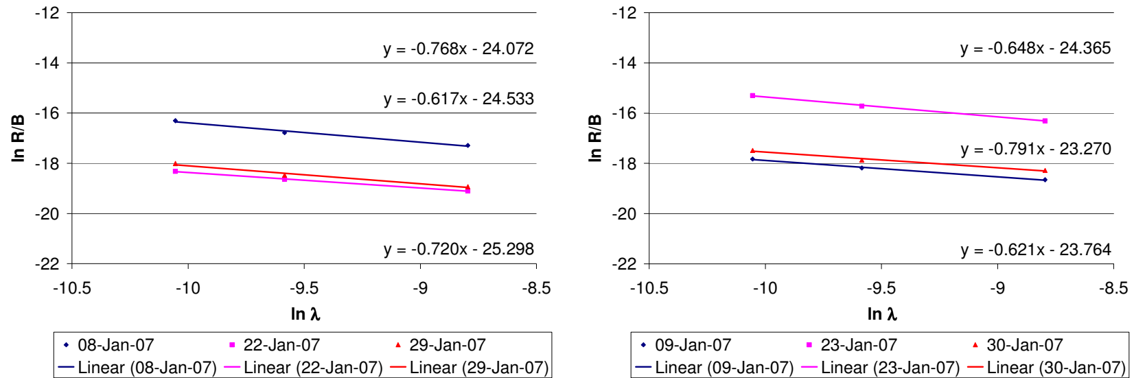
Figure 83: \ln R/B vs. \ln \lambda_{\text{eff}} plots for Krypton of INET/AVR pebbles in cycle 07-01
