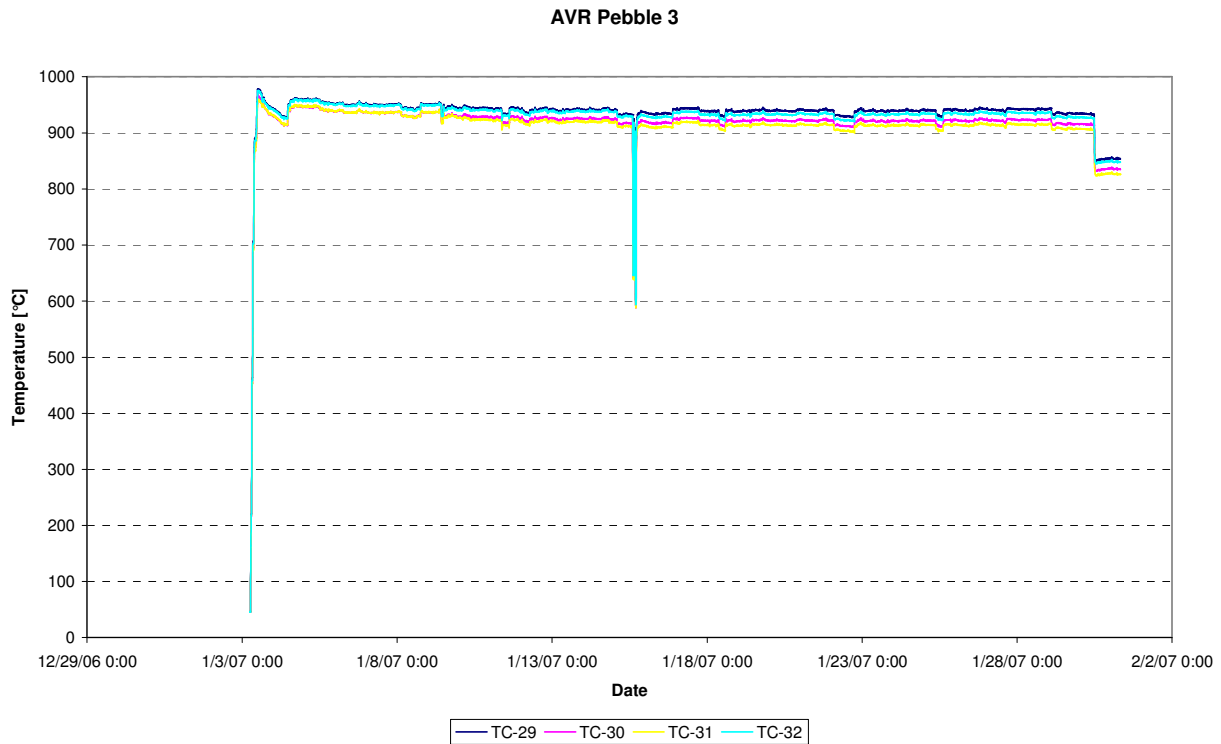
Figure 59: Temperatures pebble AVR.3 (TC-29, TC-30, TC-31, TC-32), cycle 07-01
