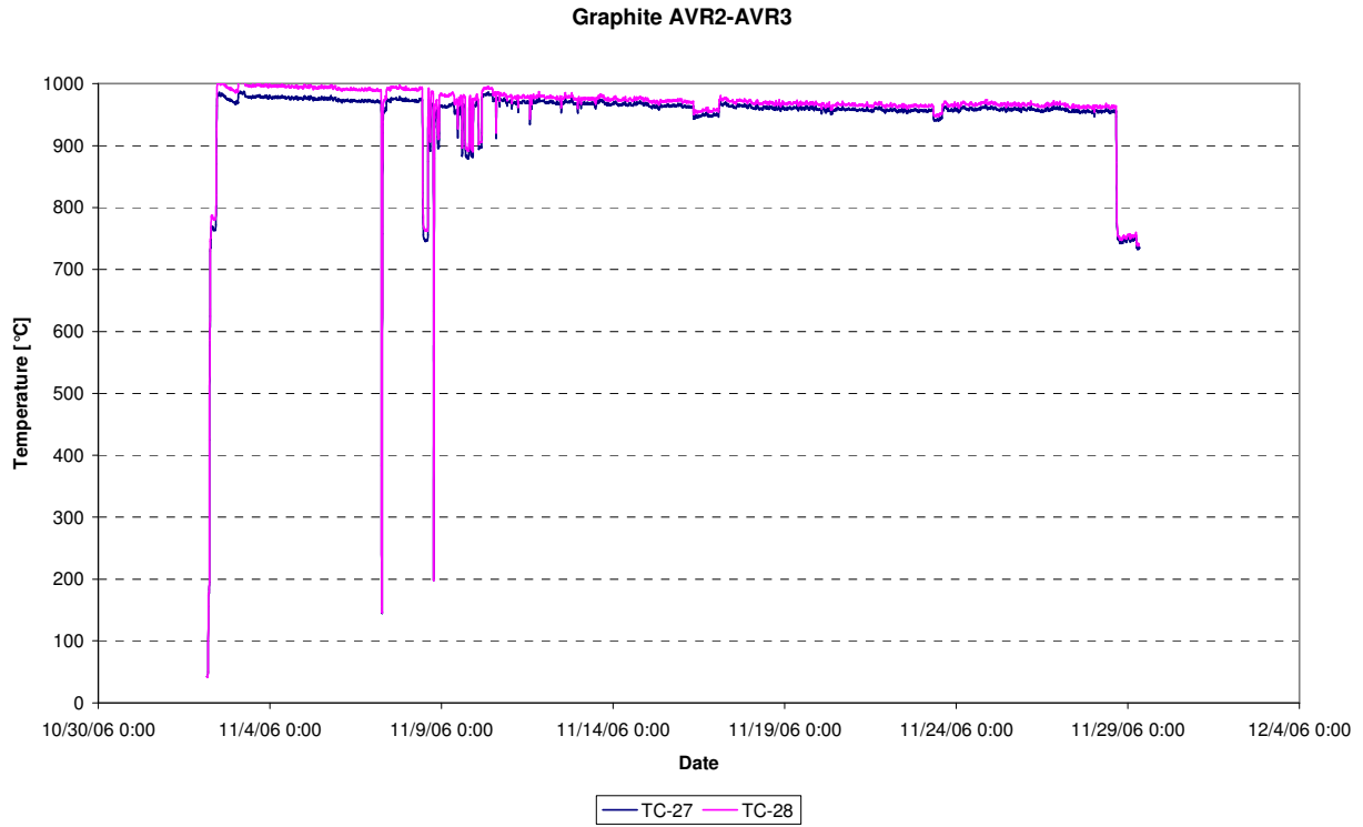
Figure 41: Temperatures graphite between AVR.2 and AVR.3 (TC-27, TC-28), cycle 06-09
