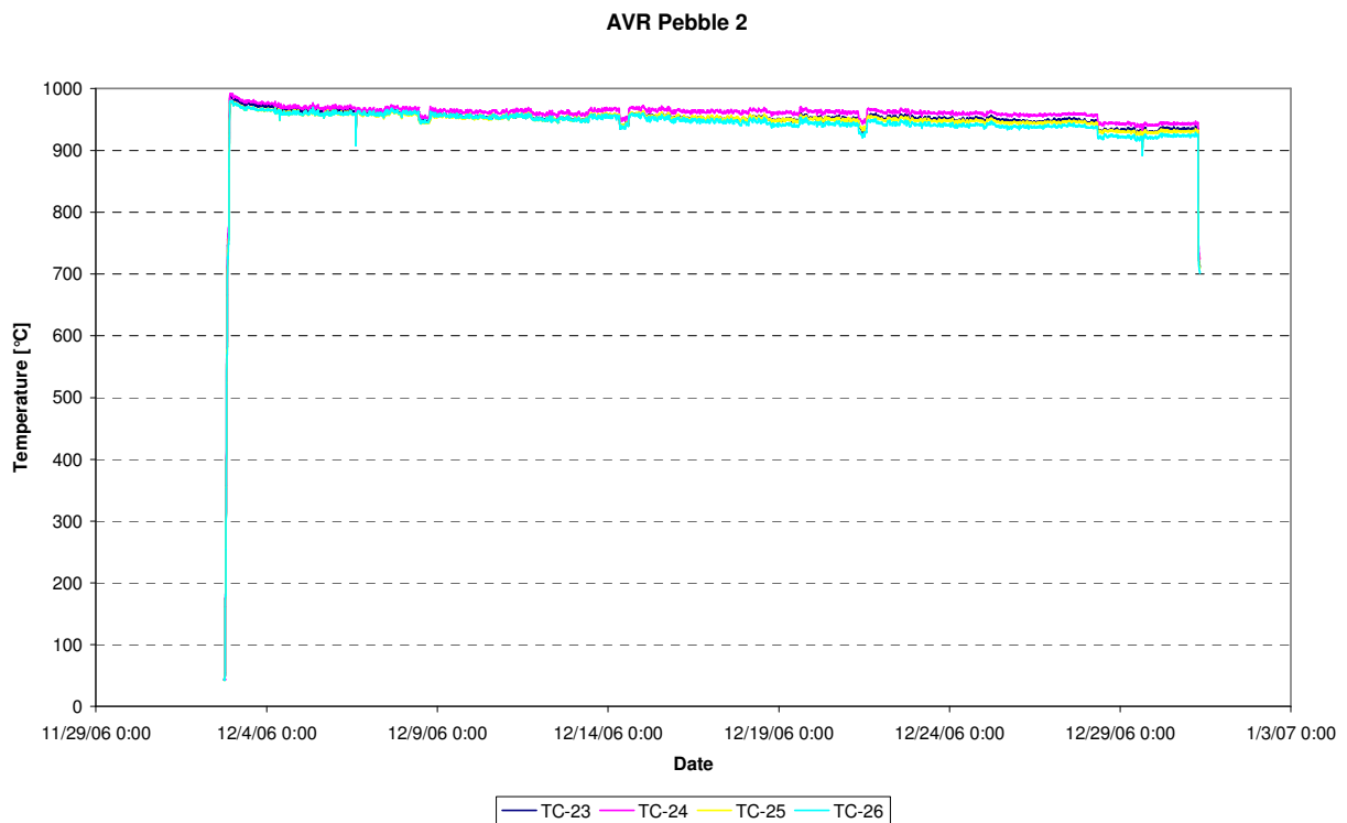
Figure 46: Temperatures pebble AVR.2 (TC-23, TC-24, TC-25, TC-26), cycle 06-10
