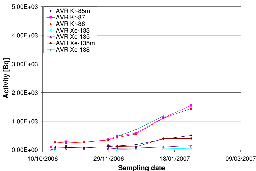
Figure 74: Purged release measurement vs. date for AVR pebbles
