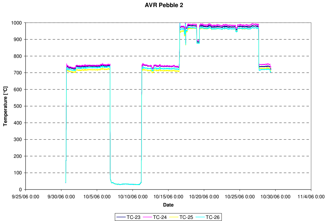
Figure 22: Temperatures pebble AVR.2 (TC-23, TC-24, TC-25, TC-26), cycle 06-08
