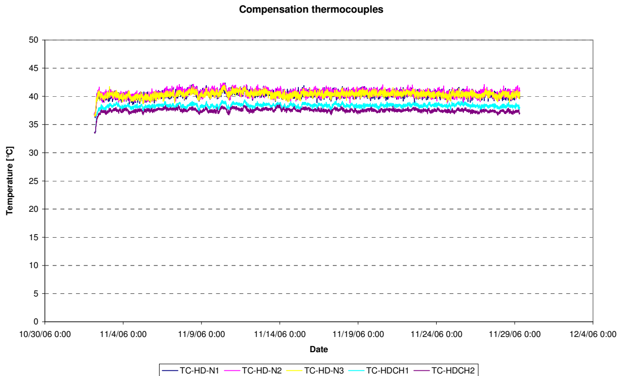
Figure 68: Reference thermocouples for temperatures compensation cycle 06-09
