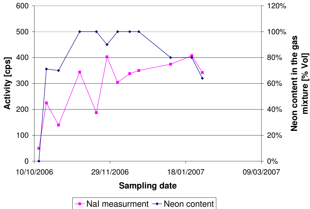
Figure 89: Correlation of NaI and Neon content in gas mixture for INET pebbles
