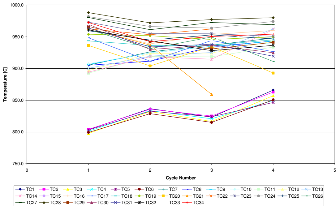
Figure 18: Evolution of average temperatures during irradiation
