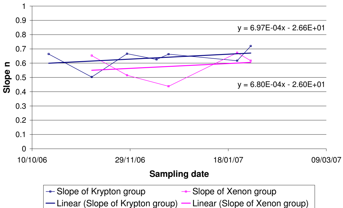
Figure 85: Evolution of the slope through time for INET pebbles
