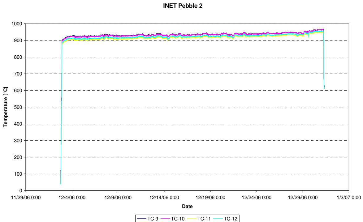
Figure 44: Temperatures pebble INET.2 (TC-09, TC-10, TC-11, TC-12), cycle 06-10
