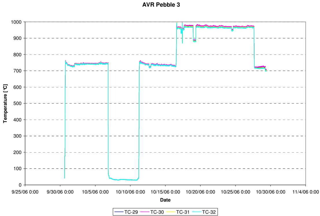
Figure 23: Temperatures pebble AVR.3 (TC-29, TC-30, TC-31, TC-32), cycle 06-08
