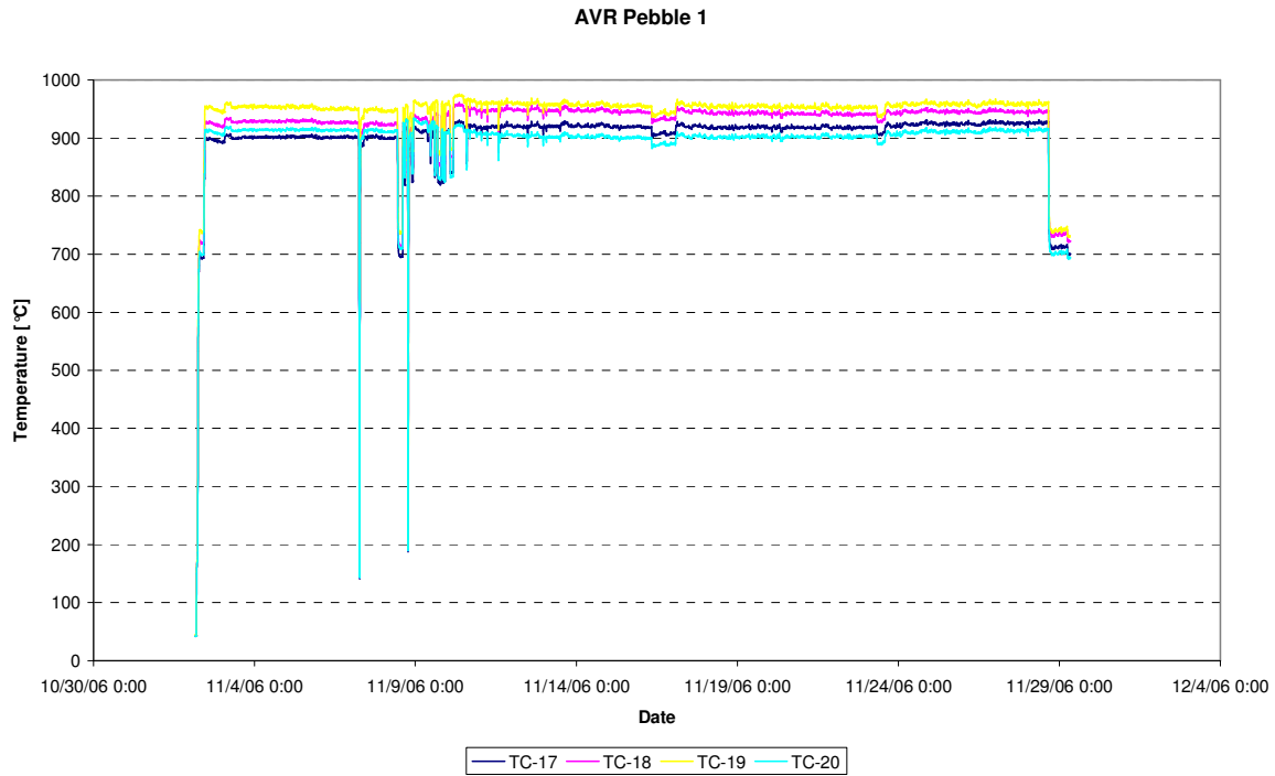
Figure 33: Temperatures pebble AVR.1 (TC-17, TC-18, TC-19, TC-20), cycle 06-09
