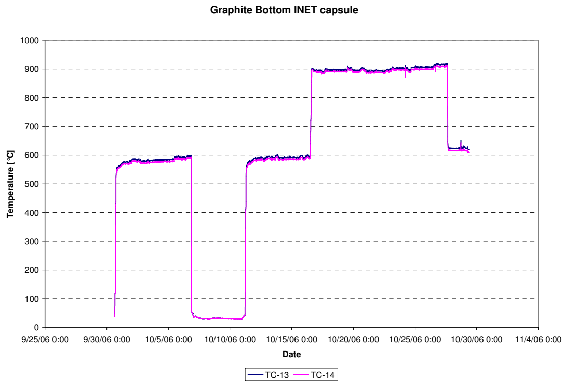
Figure 26: Temperatures bottom graphite INET Capsule (TC-13, TC-14), cycle 06-08
