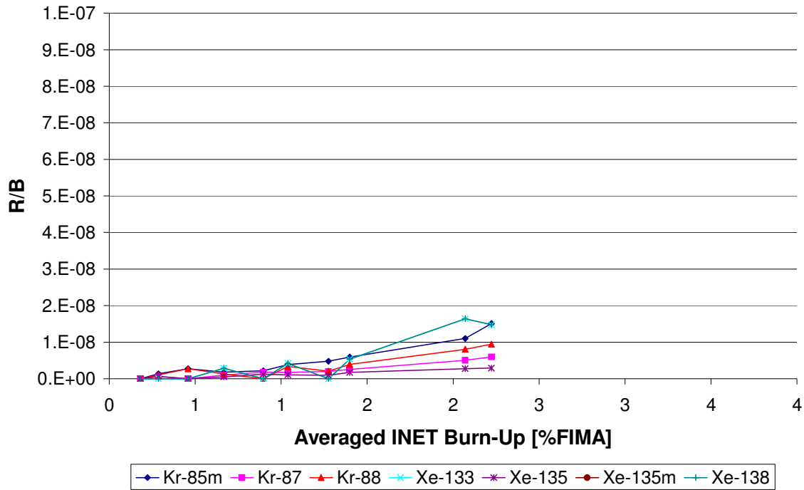
Figure 75: R/B vs. burnup for INET pebbles
