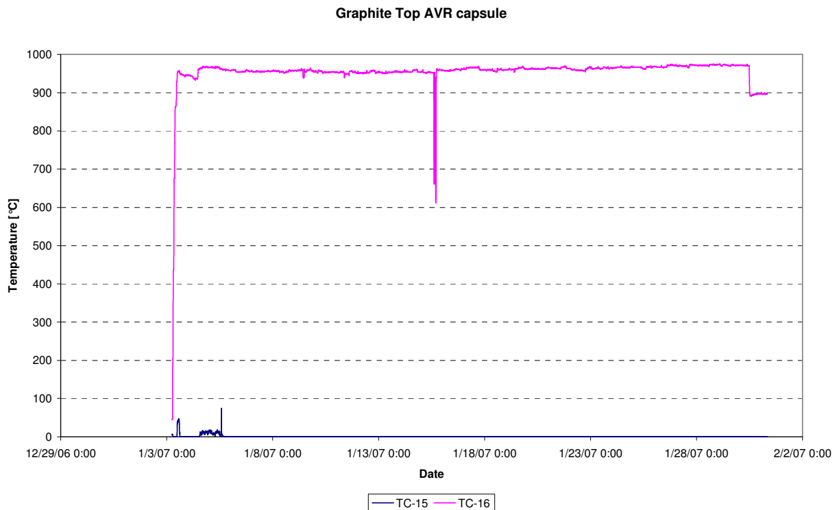
Figure 63: Temperatures top graphite AVR capsule (TC-15, TC-16), cycle 07-01
