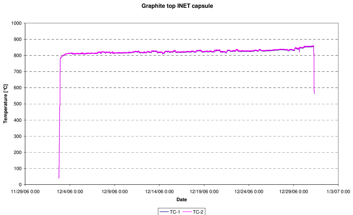
Figure 48: Temperatures top graphite INET capsule (TC-01, TC-02), cycle 06-10
