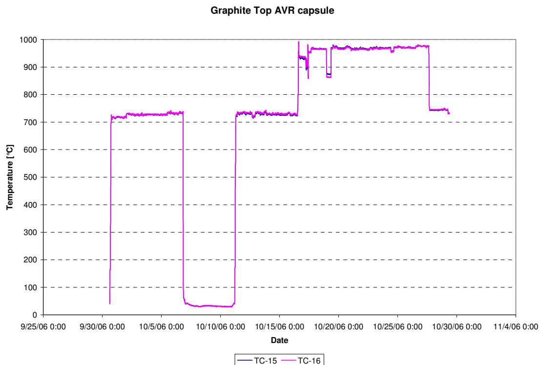
Figure 27: Temperatures top graphite AVR capsule (TC-15, TC-16), cycle 06-08
