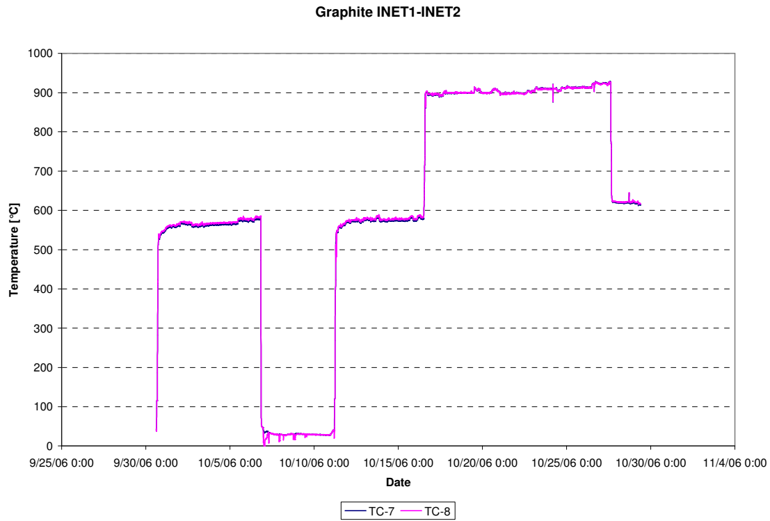
Figure 25: Temperatures graphite between INET.1 and INET.2 (TC-07, TC-08), cycle 06-08
