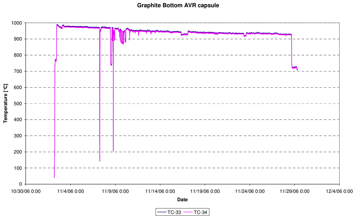
Figure 42: Temperatures bottom graphite (TC-33, TC-34), cycle 06-09
