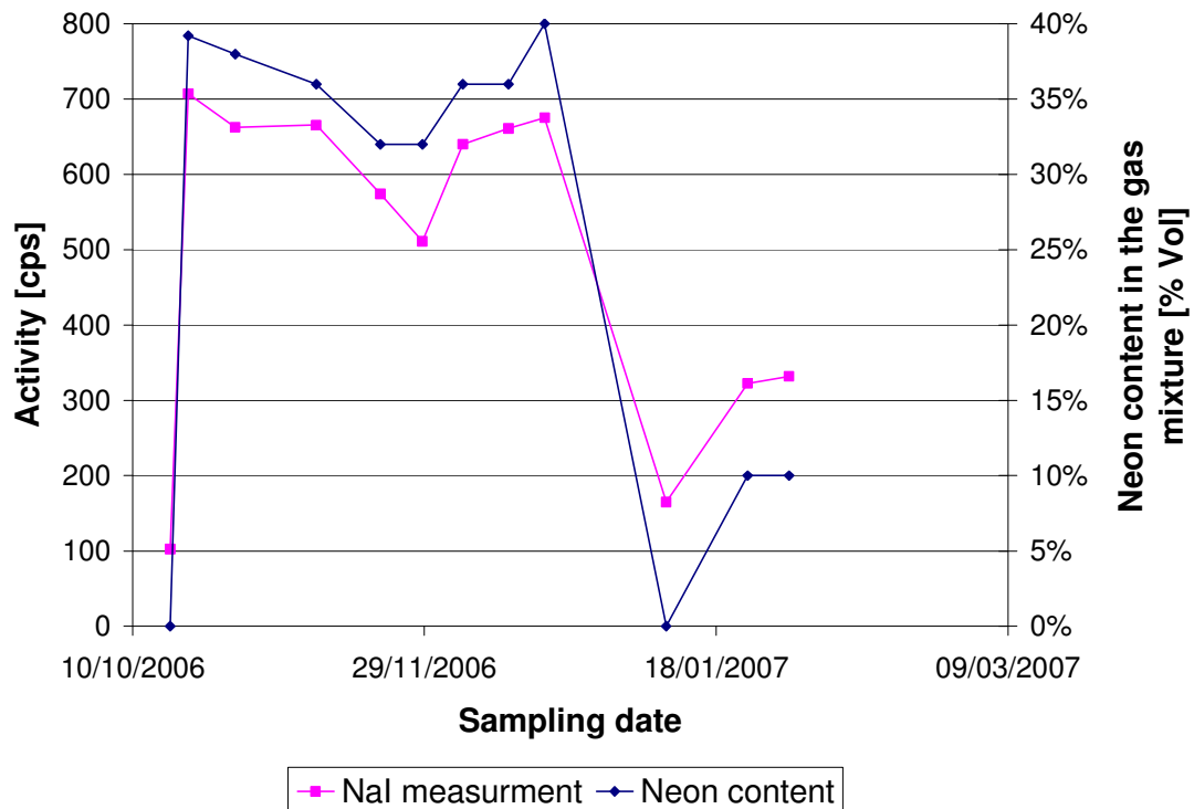
Figure 90: Correlation of NaI and Neon content in gas mixture for AVR pebbles
