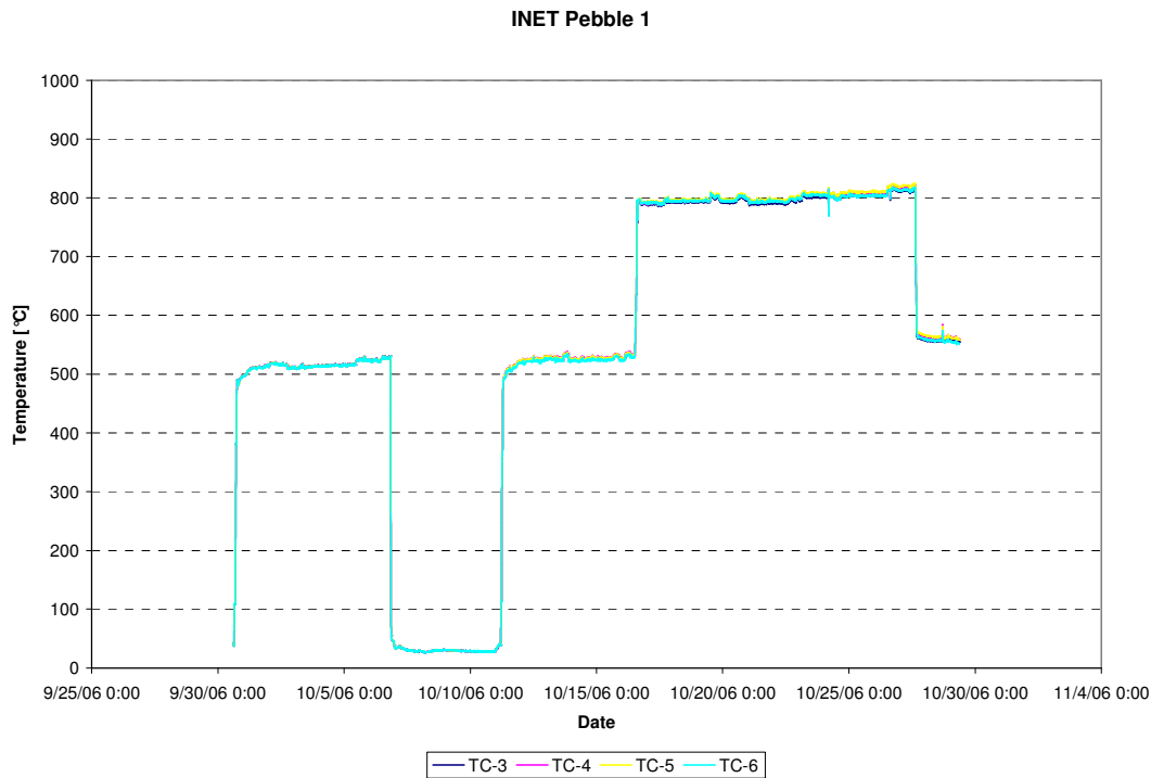
Figure 19: Temperatures pebble INET.1 (TC-03, TC-04, TC-05, TC-06), cycle 06-08
