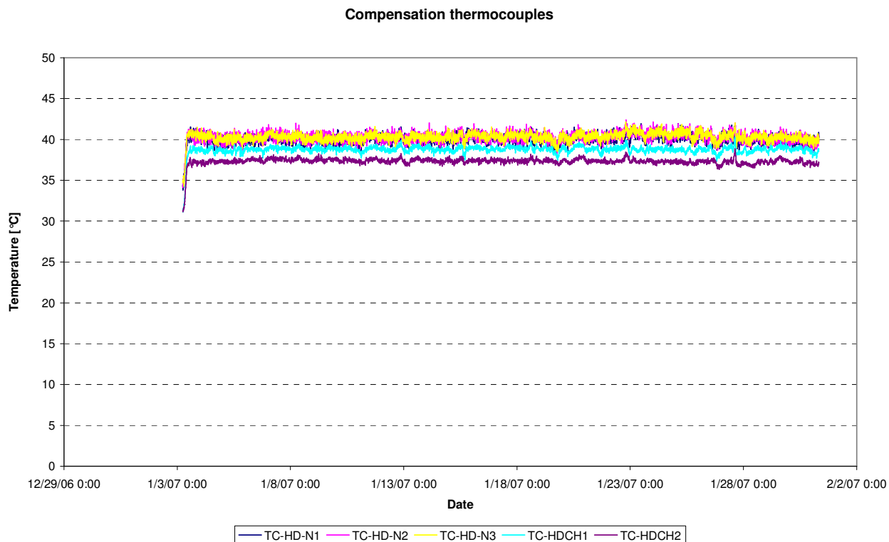
Figure 70: Reference thermocouples for temperatures compensation cycle 07-01
