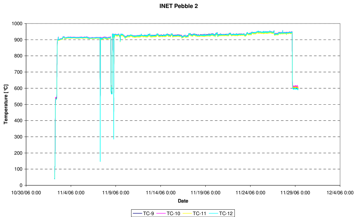
Figure 32: Temperatures pebble INET.2 (TC-09, TC-10, TC-11, TC-12), cycle 06-09
