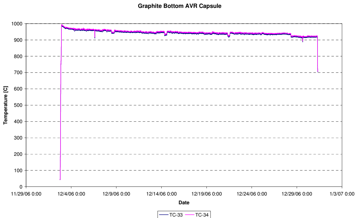
Figure 54: Temperatures bottom graphite (TC-33, TC-34), cycle 06-10
