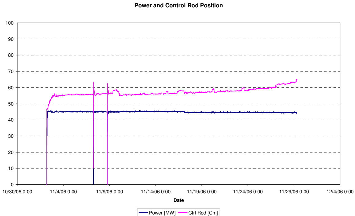
Figure 6: Reactor Power/Control Rod position cycle 06-09
