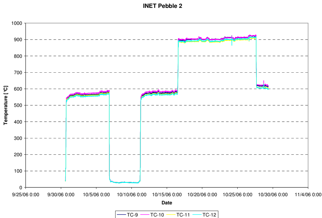
Figure 20: Temperatures pebble INET.2 (TC-09, TC-10, TC-11, TC-12), cycle 06-08
