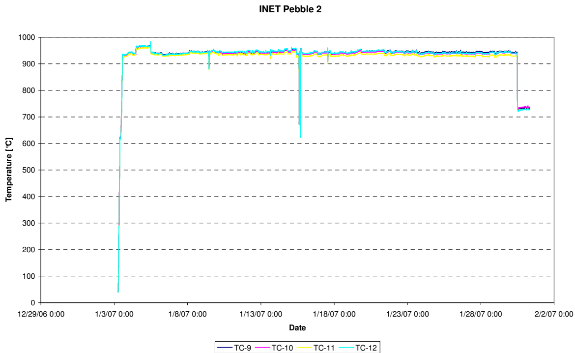
Figure 56: Temperatures pebble INET.2 (TC-09, TC-10, TC-11, TC-12), cycle 07-01
