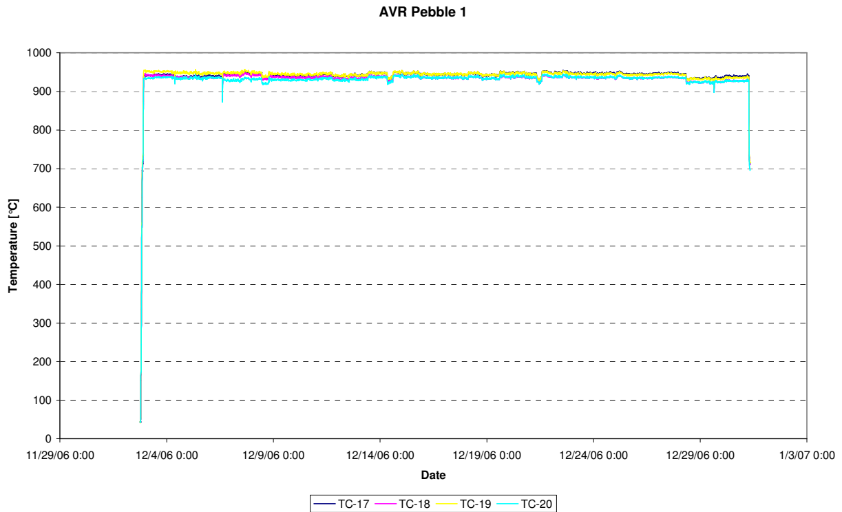
Figure 45: Temperatures pebble AVR.1 (TC-17, TC-18, TC-19, TC-20), cycle 06-10
