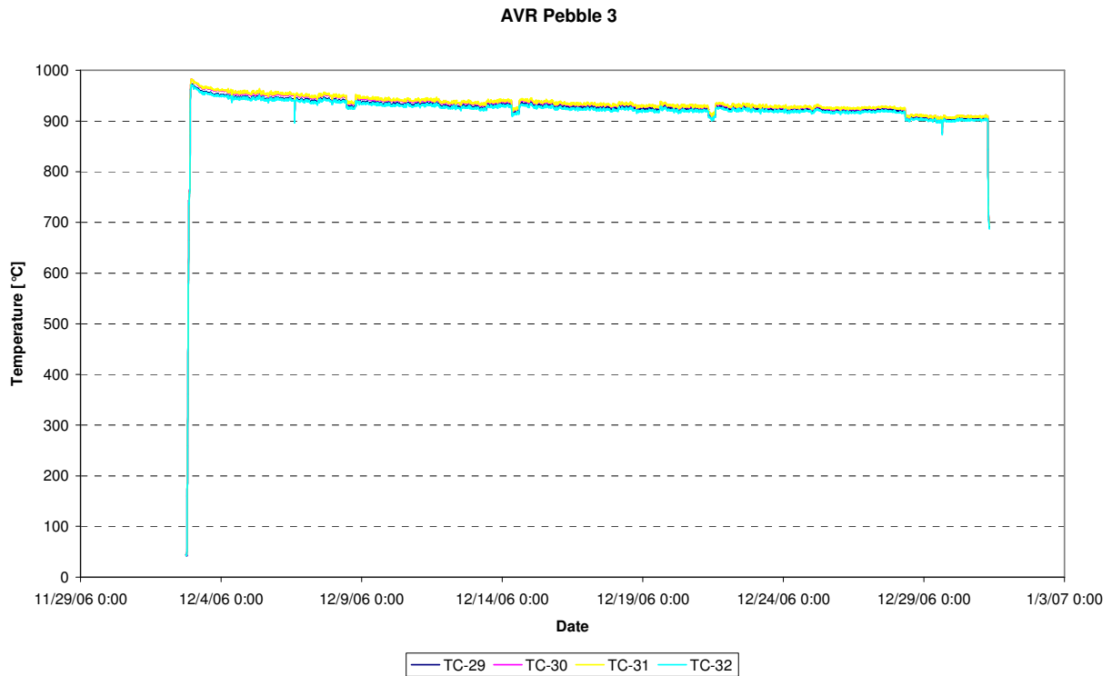
Figure 47: Temperatures pebble AVR.3 (TC-29, TC-30, TC-31, TC-32), cycle 06-10
