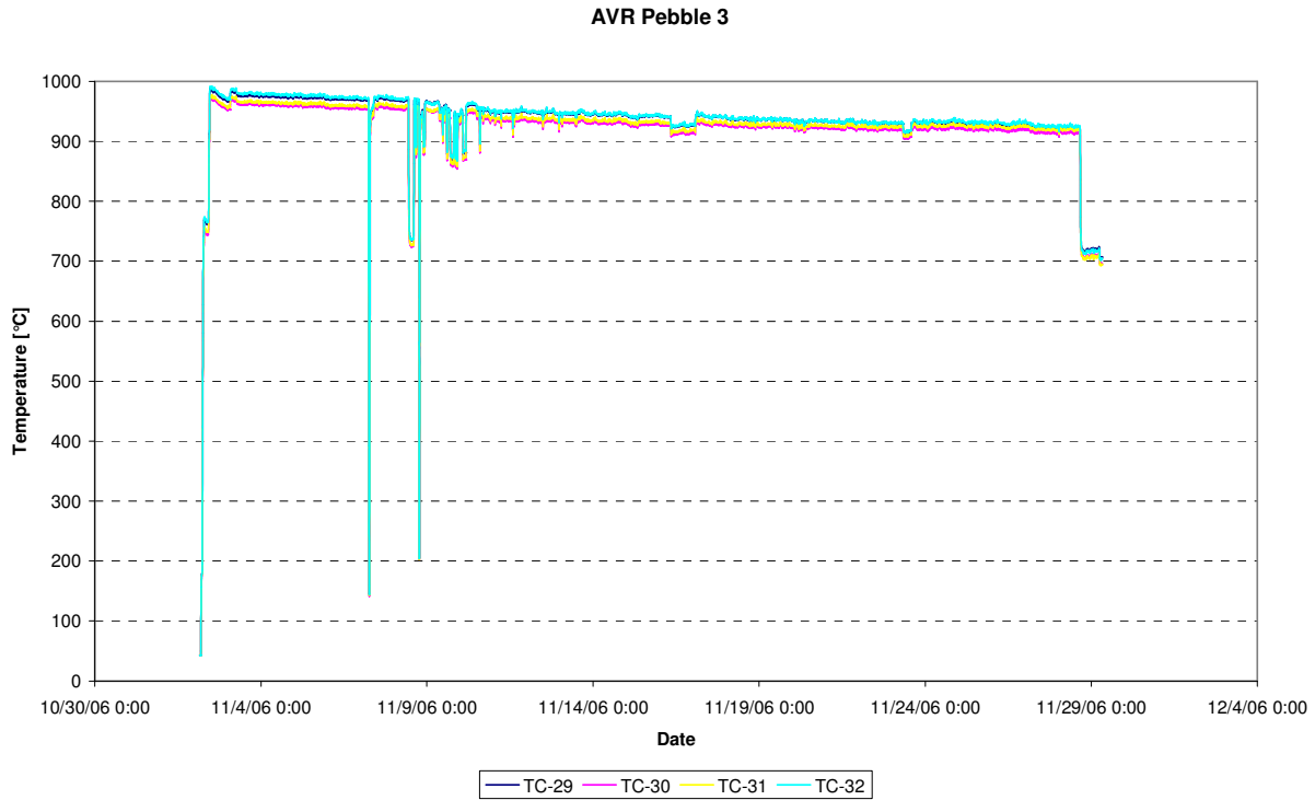
Figure 35: Temperatures pebble AVR.3 (TC-29, TC-30, TC-31, TC-32), cycle 06-09
