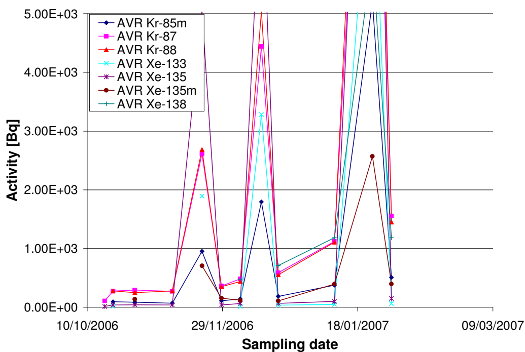
Figure 72: Release measurement vs. date for AVR pebbles
