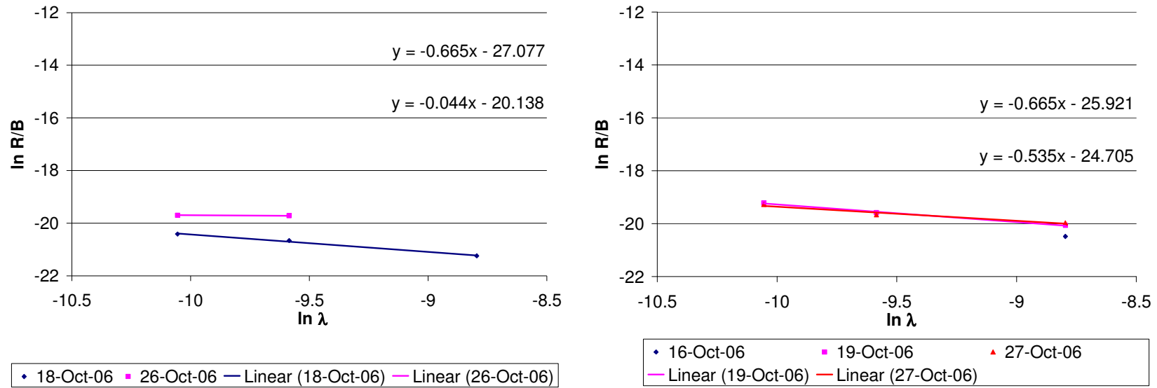
Figure 77: \ln R/B vs. \ln \lambda_{\text{eff}} plots for Krypton of INET/AVR pebbles in cycle 06-08
