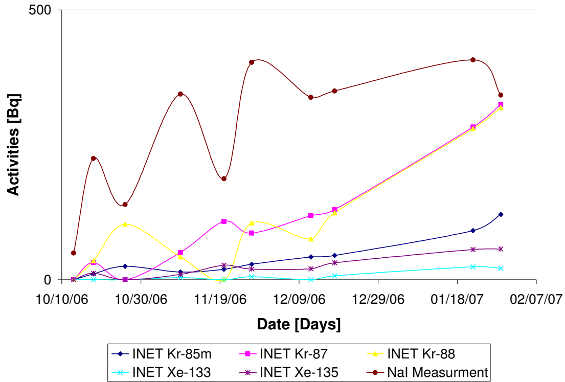
Figure 87: Nal and Gamma spectrometer measurements correlation for INET pebbles
