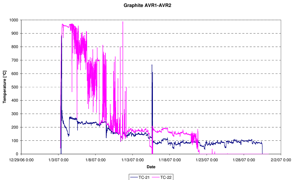
Figure 64: Temperatures graphite between AVR.1 and AVR.2 (TC-21, TC-22), cycle 07-01
