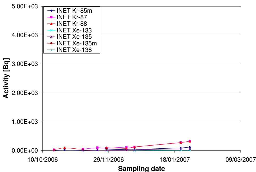
Figure 73: Purged release measurement vs. date for INET pebbles
