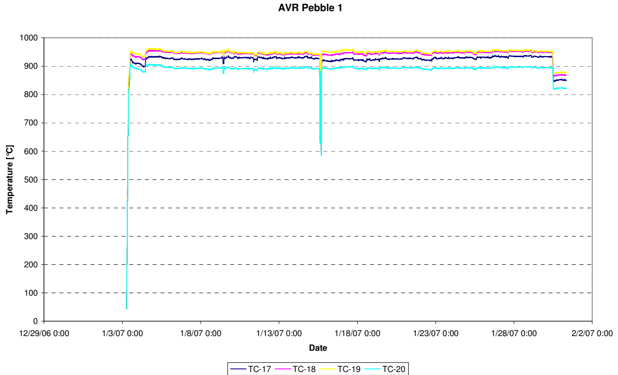
Figure 57: Temperatures pebble AVR.1 (TC-17, TC-18, TC-19, TC-20), cycle 07-01
