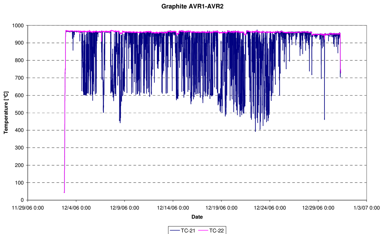
Figure 52: Temperatures graphite between AVR.1 and AVR.2 (TC-21, TC-22), cycle 06-10
