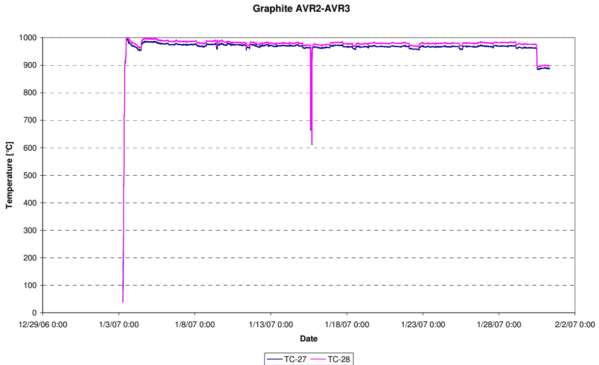
Figure 65: Temperatures graphite between AVR.2 and AVR.3 (TC-27, TC-28), cycle 07-01
