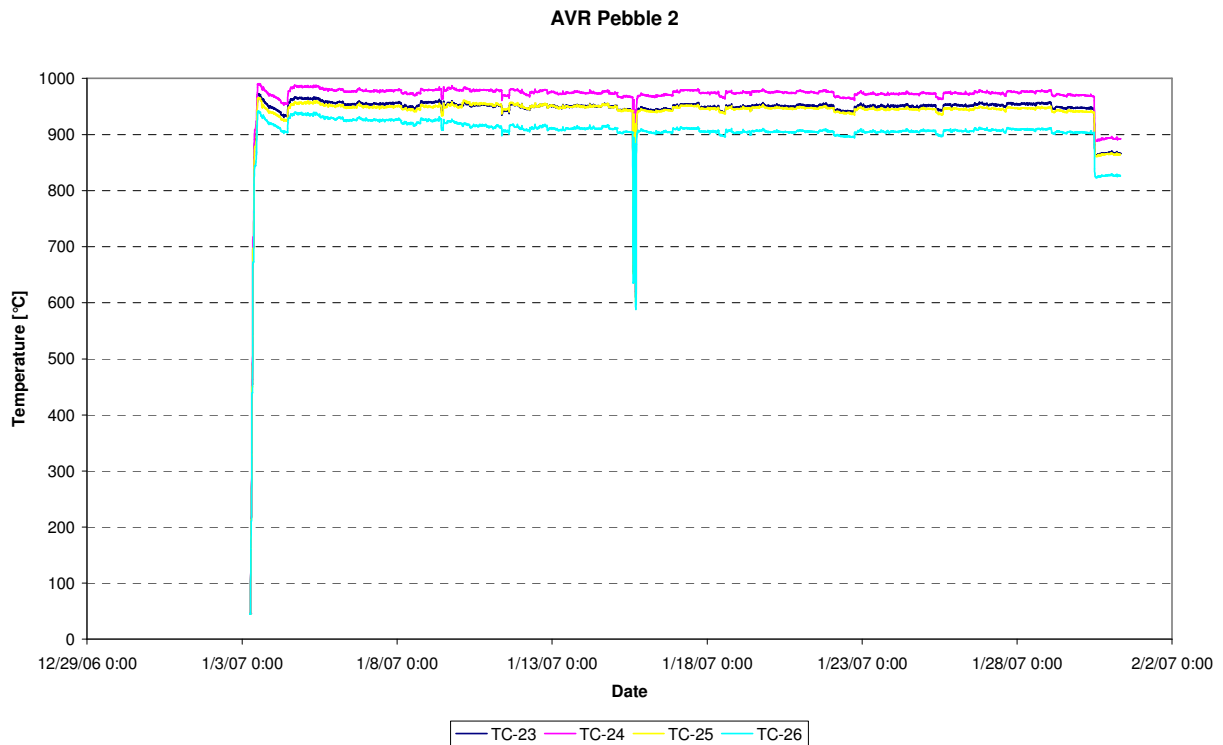
Figure 58: Temperatures pebble AVR.2 (TC-23, TC-24, TC-25, TC-26), cycle 07-01
