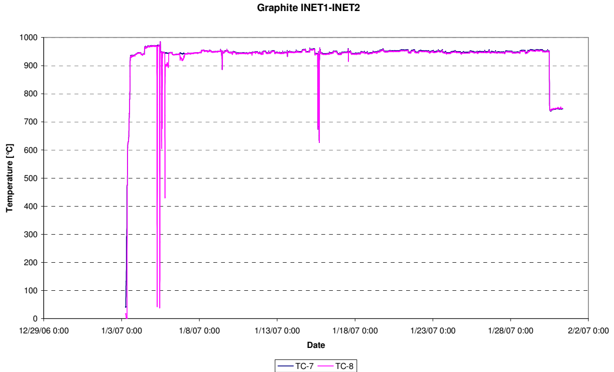
Figure 61: Temperatures graphite between INET.1 and INET.2 (TC-07, TC-08), cycle 07-01
