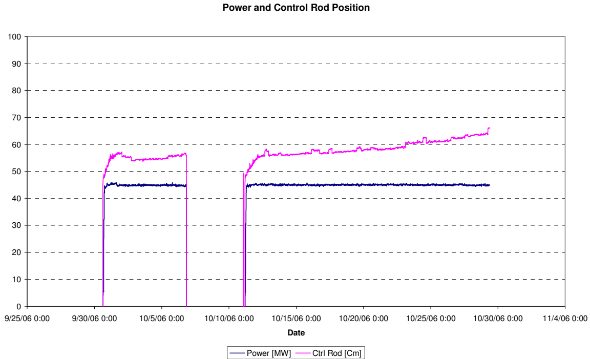
Figure 5: Reactor Power/Control Rod position cycle 06-08
