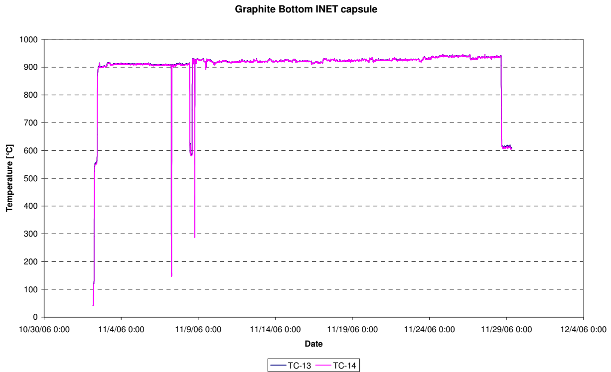
Figure 38: Temperatures bottom graphite INET Capsule (TC-13, TC-14), cycle 06-09
