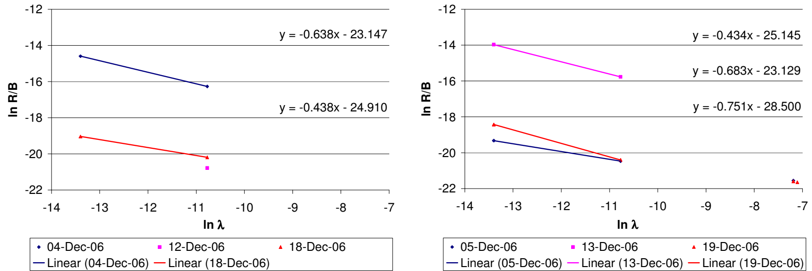
Figure 82: \ln R/B vs. \ln \lambda_{\text{eff}} plots for Xenon of INET/AVR pebbles in cycle 06-10
