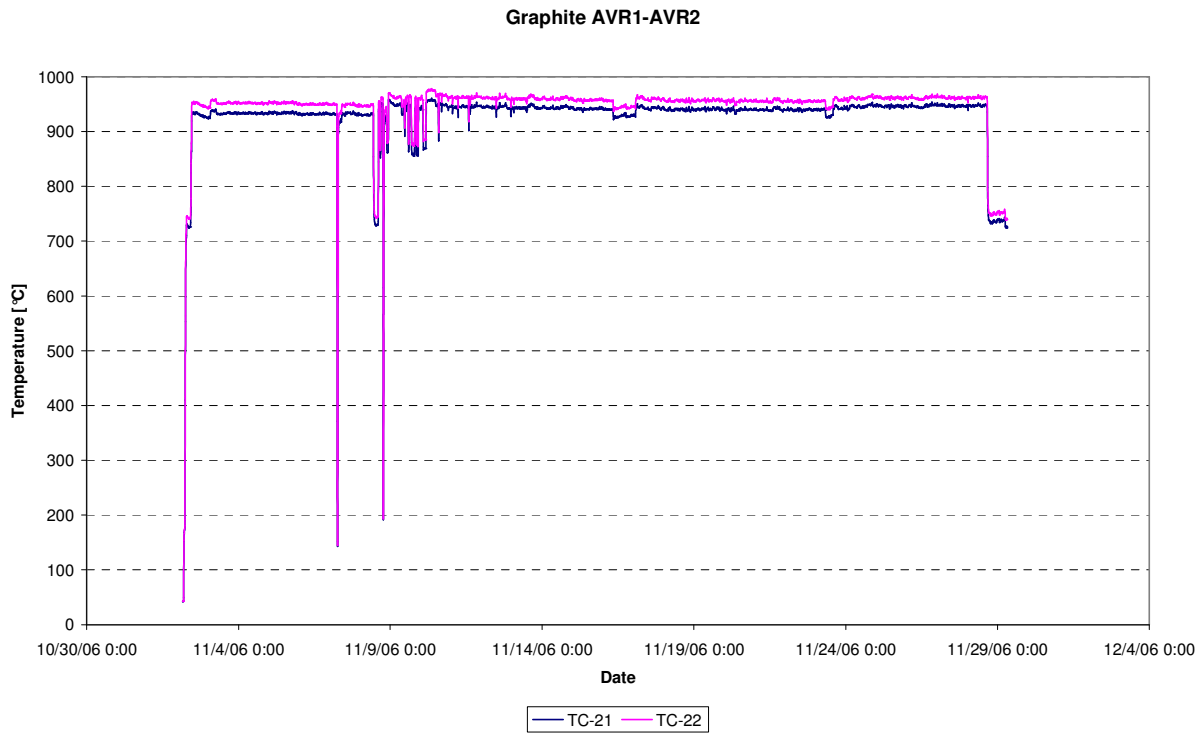
Figure 40: Temperatures graphite between AVR.1 and AVR.2 (TC-21, TC-22), cycle 06-09
