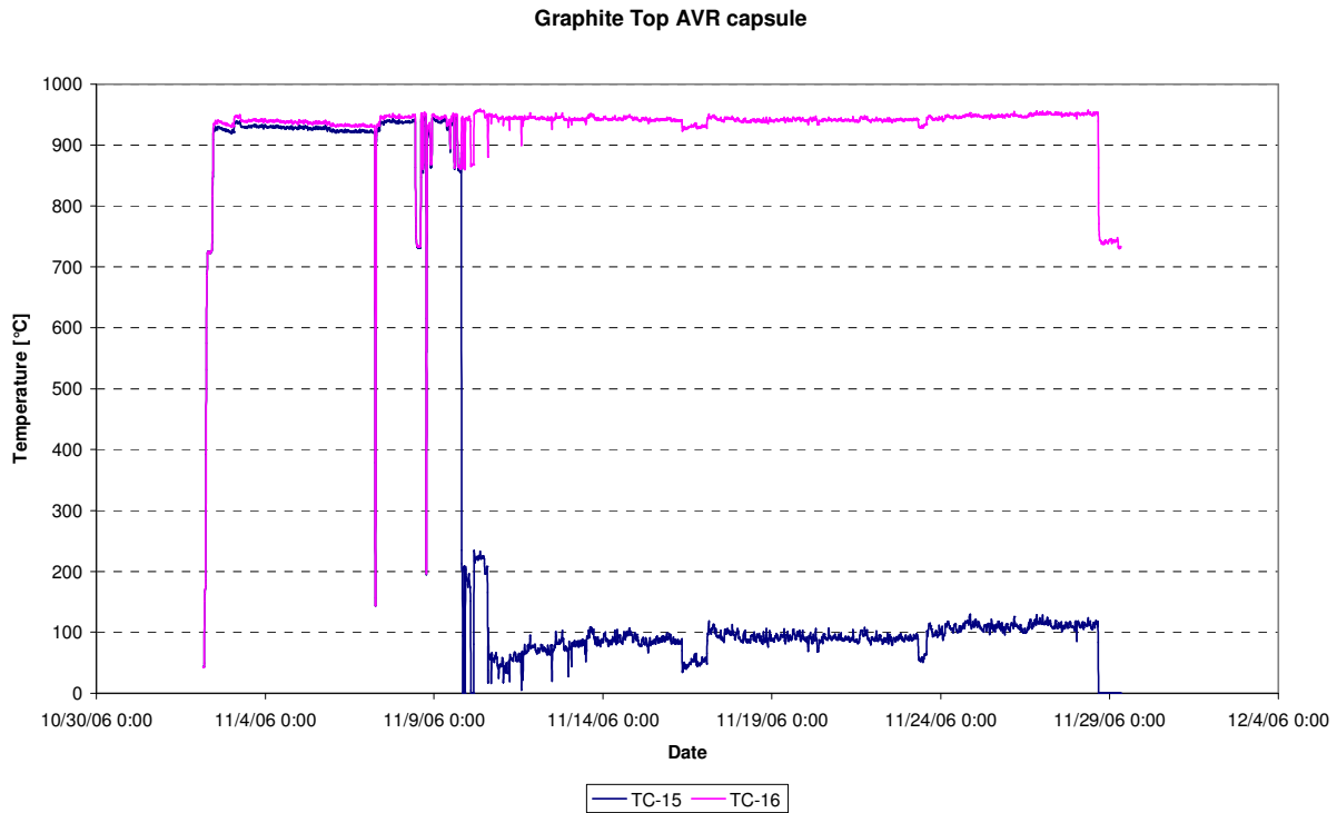
Figure 39: Temperatures top graphite AVR capsule (TC-15, TC-16), cycle 06-09
