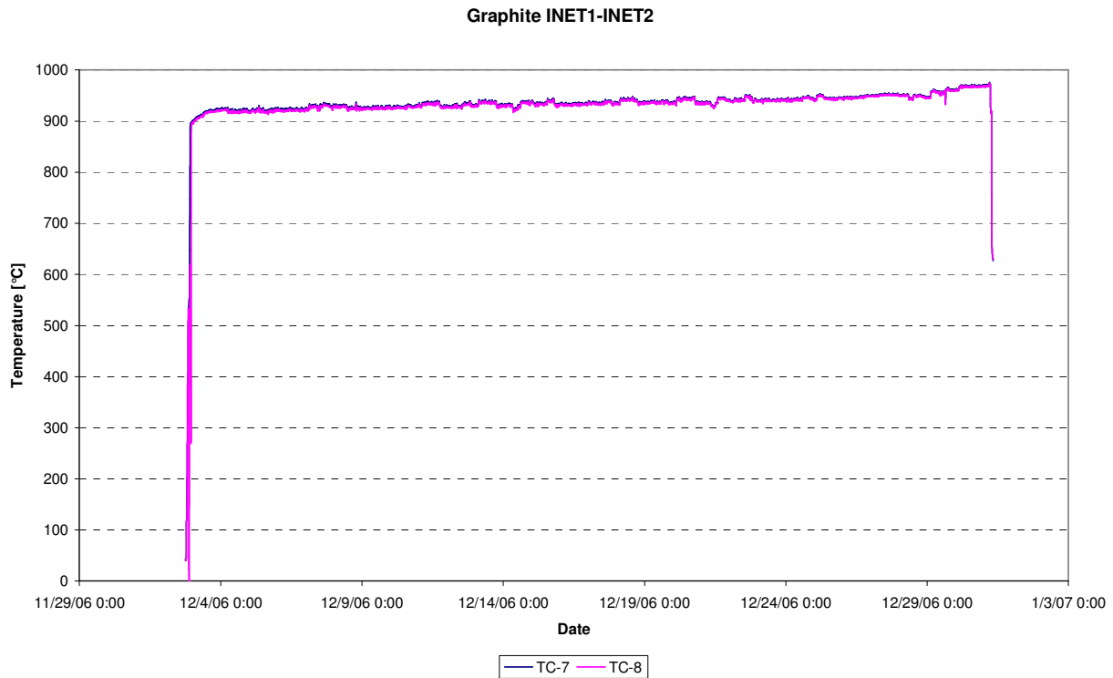
Figure 49: Temperatures graphite between INET.1 and INET.2 (TC-07, TC-08), cycle 06-10
