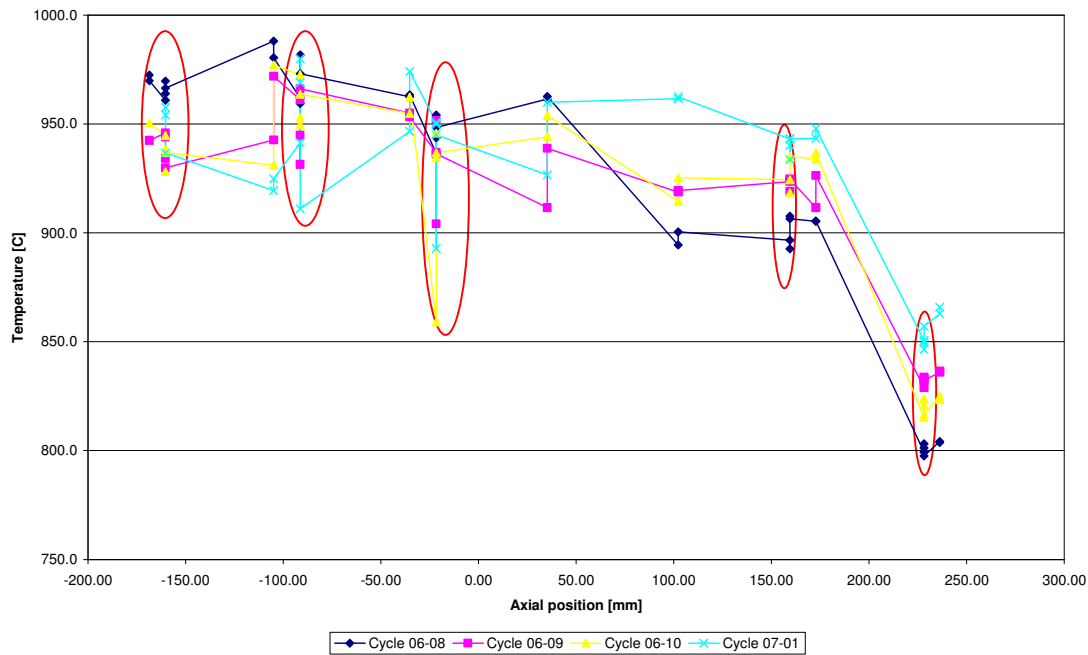
Figure 17: Average temperatures in irradiation rig for all 4 irradiation cycles
