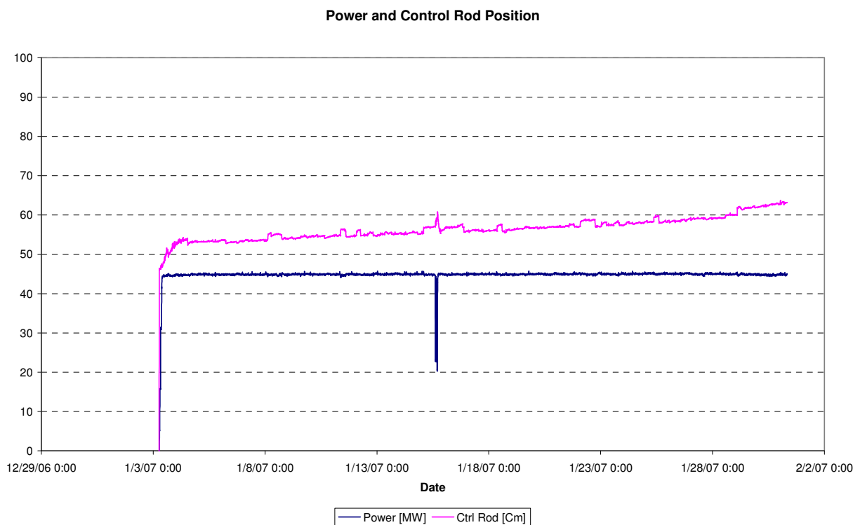
Figure 8: Reactor Power/Control Rod position cycle 07-01
