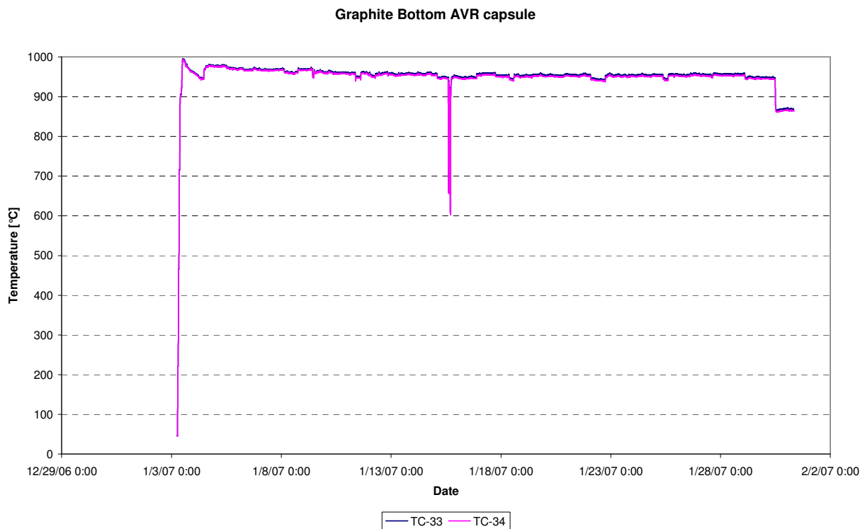
Figure 66: Temperatures bottom graphite (TC-33, TC-34), cycle 07-01
