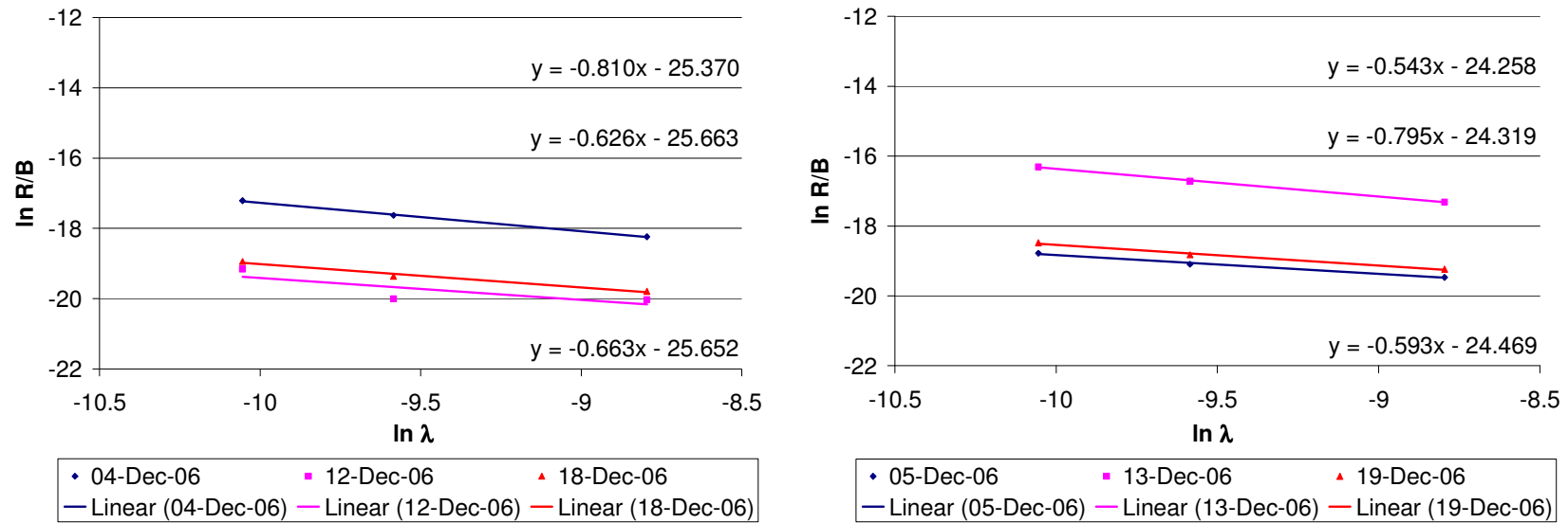
Figure 81: \ln R/B vs. \ln \lambda_{\text{eff}} plots for Krypton of INET/AVR pebbles in cycle 06-10
