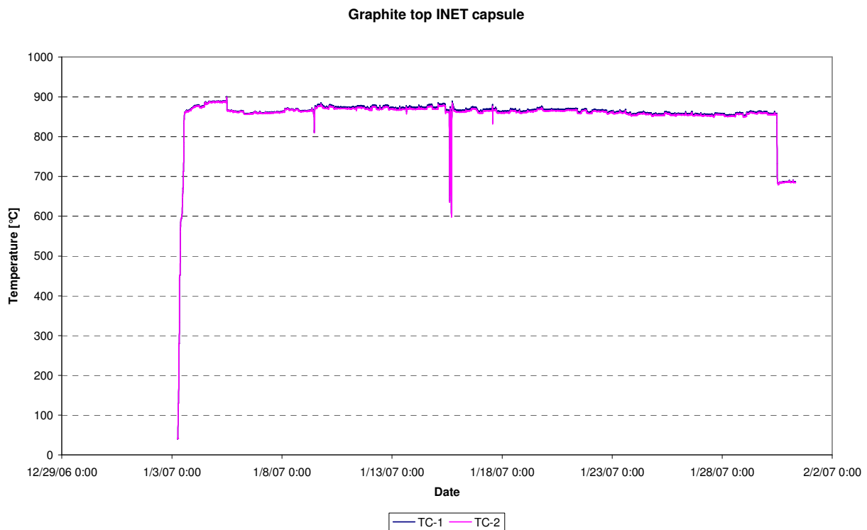
Figure 60: Temperatures top graphite INET capsule (TC-01, TC-02), cycle 07-01
