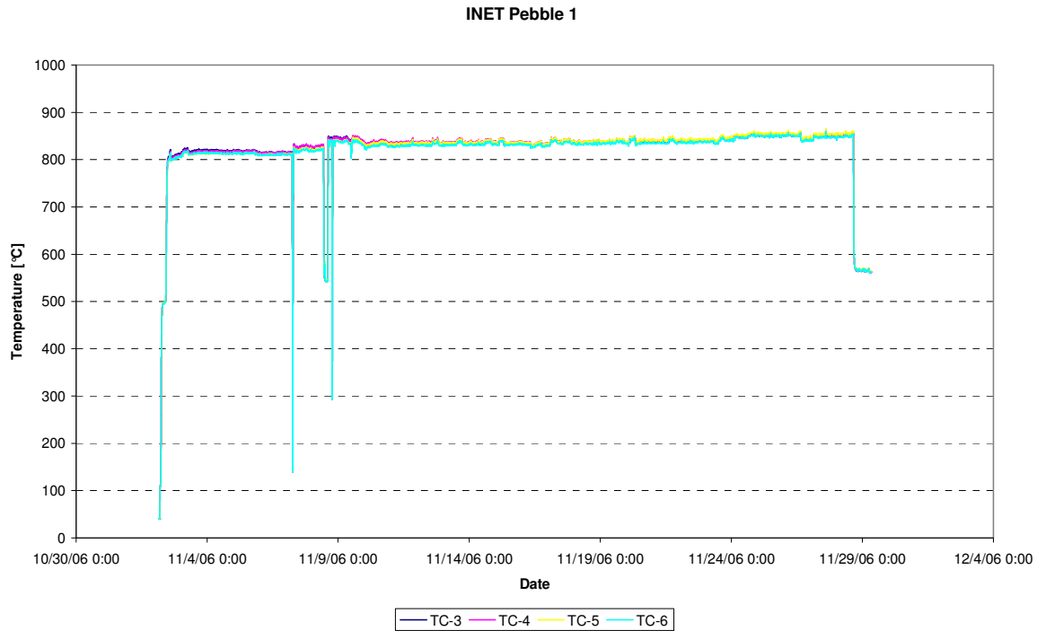
Figure 31: Temperatures pebble INET.1 (TC-03, TC-04, TC-05, TC-06), cycle 06-09
