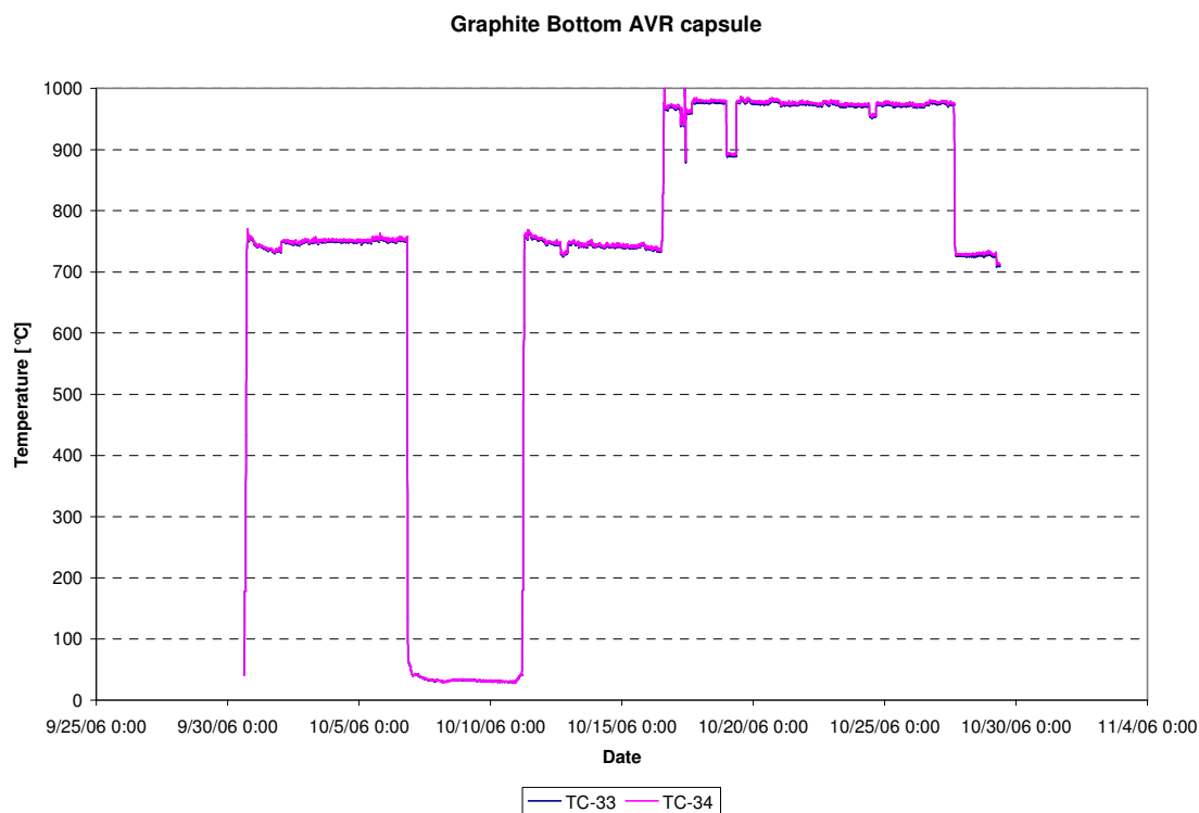
Figure 30: Temperatures bottom graphite (TC-33, TC-34), cycle 06-08
