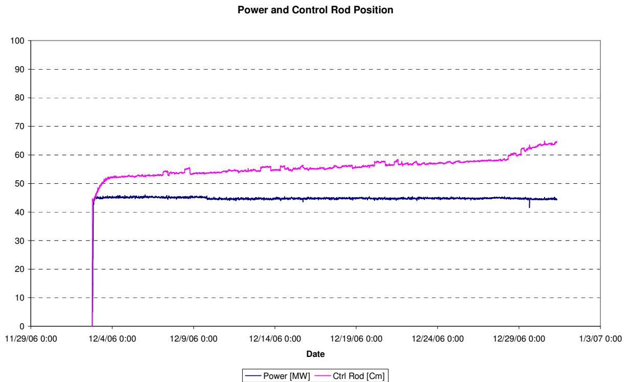
Figure 7: Reactor Power/Control Rod position cycle 06-10
