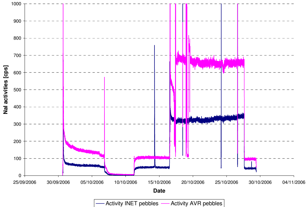
Figure 13: Nal readings cycle 06-08
