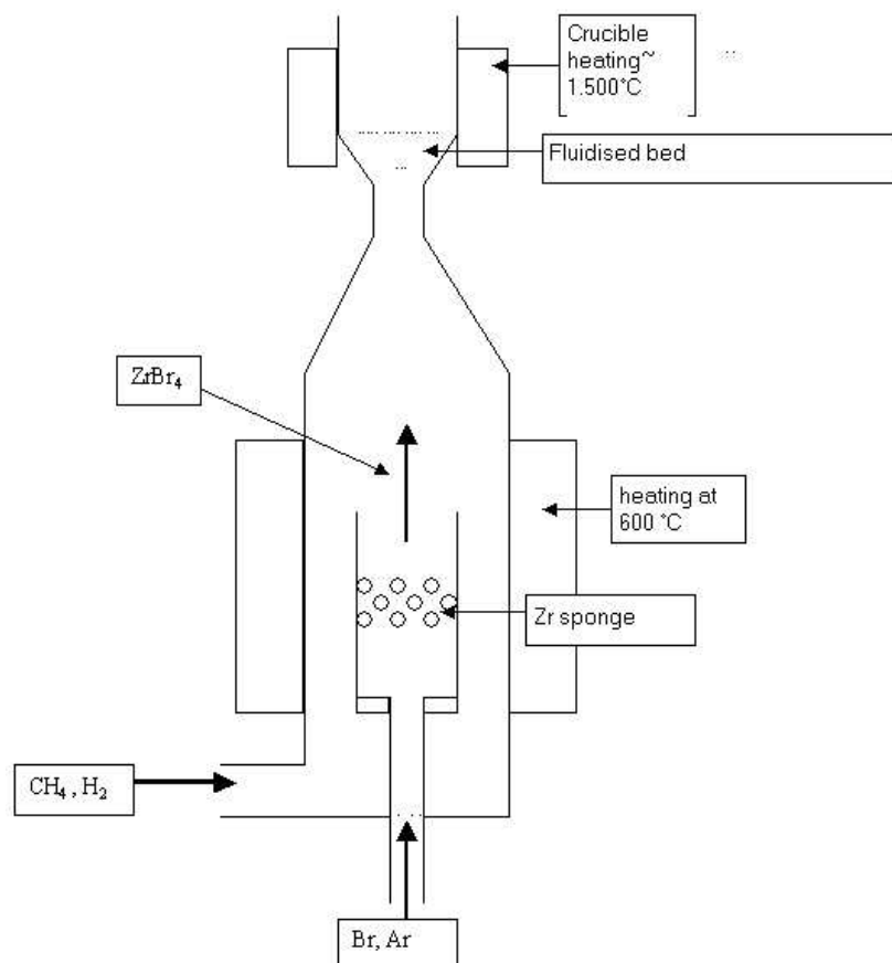
Figure I.2: Diagram of ZrC deposition using bromide installation (JAERI).
