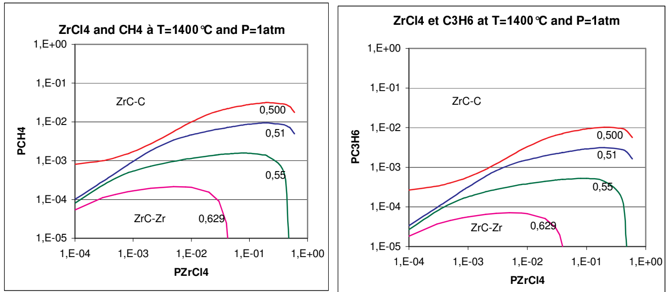
Figure II.15: Comparison of deposition graphs for \text{CH}_4 and \text{C}_3\text{H}_6 .
