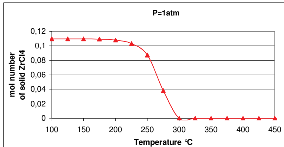
Figure II.16: Condensation of the \text{ZrCl}_4 formed during chlorination.
