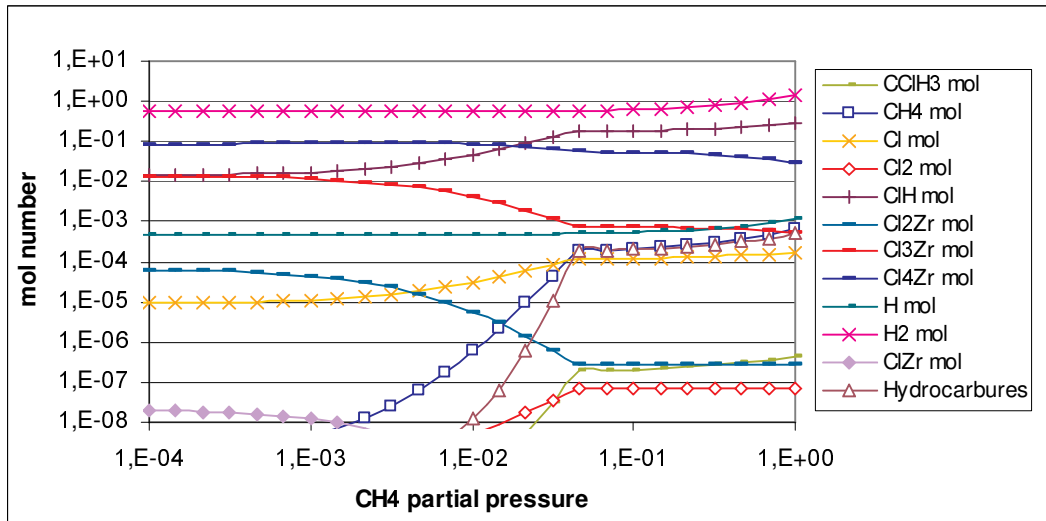
Figure II.13: Composition of the gaseous phase at T=1,600^{\circ}\text{C} and P_{\text{ZrCl}_4}=0.1 atm.
