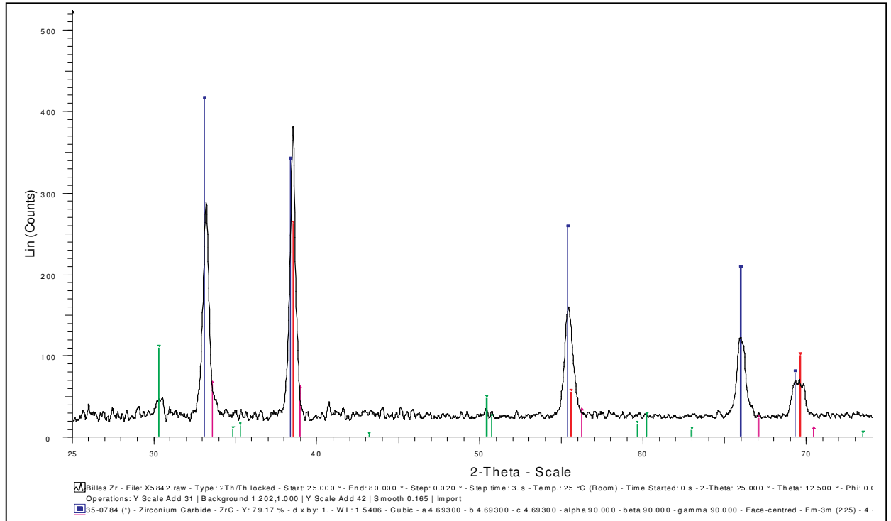
Figure IV.3: Deposition spectrum obtained by XRD.
