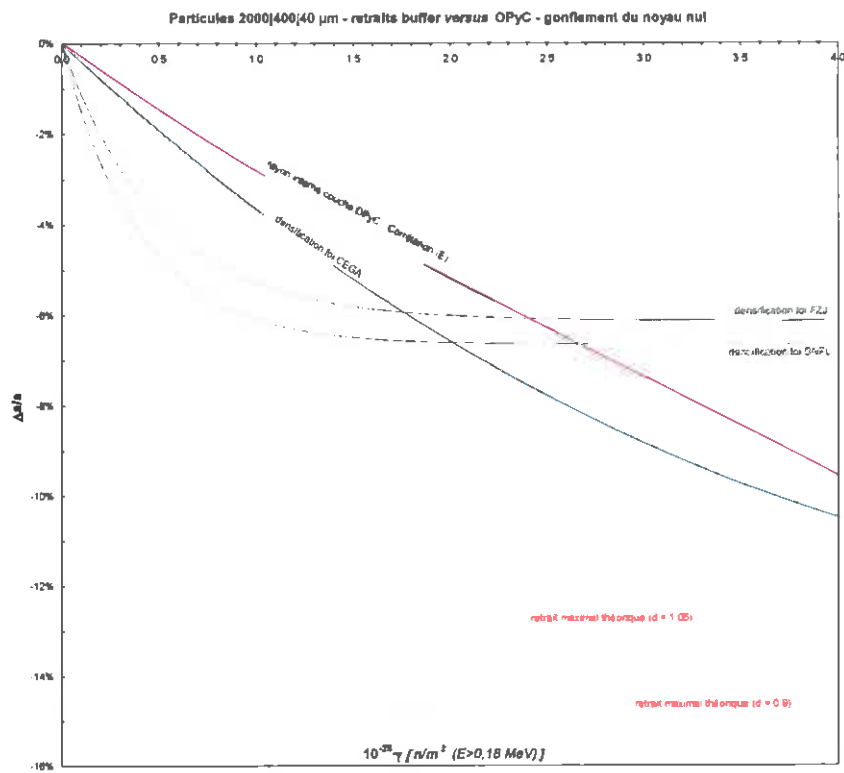
FIGURE 9: BUFFER SHRINKAGE VERSUS OPyC – 2000/400 \mu\text{m}
