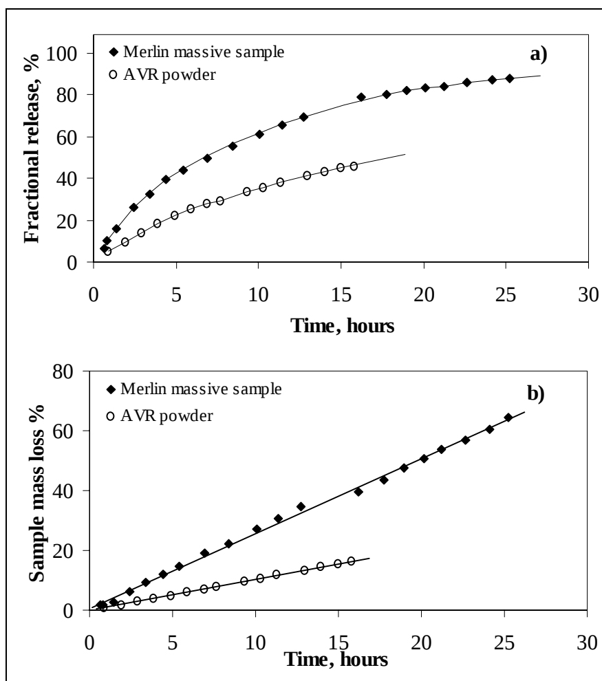
Figure 4.5: ^{14}\text{C} release (a) and mass loss (b) during Merlin and AVR graphite oxidation with water steam (water vapor pressure 2.3 kPa)
